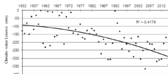
Figure 2 - Evolution of water balance from 1952 to 2015 calculated between April 1 and September 30 for the Saint-Emilion region (France).
