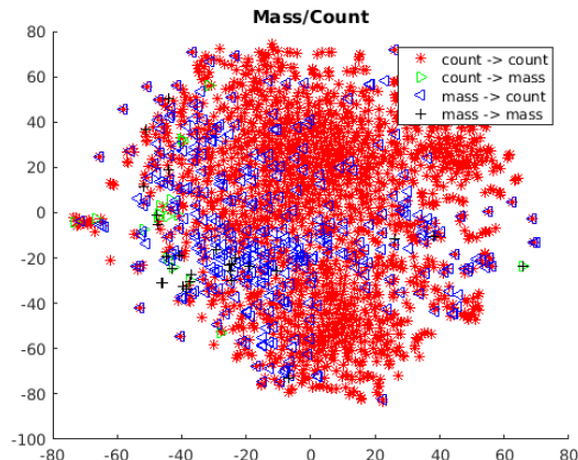
Figure 5: tSNE representation of the word vectors associated with the mass nouns and count nouns by the neural network.
