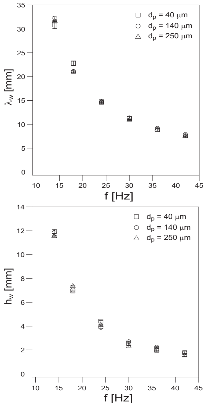
FIG. 14. The length, \lambda_w (top), and the amplitude, h_w (bottom), of the Faraday waves, measured at the onset of grains motions, as a function of the forcing frequency, f , and parameterized in d_p .
