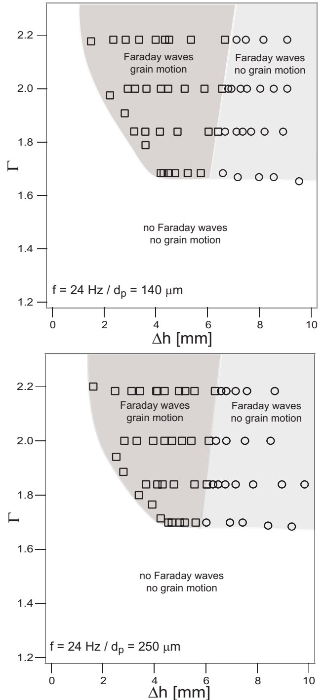
FIG. 12. Parameters plane \Gamma - \Delta h for d_p 140 \mu\text{m} (top) and 250 \mu\text{m} (bottom).
