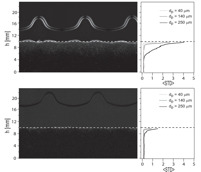
FIG. 8. Gray level Standard Deviation Map, showing active zones of moving grains in the granular bed. Top: the active layer of sedimented particles shown below de Faraday waves extend over several grain sizes ( \Delta h = 4.7 \text{ mm} ). Bottom: below the threshold (for \Delta h > \Delta h_c ) there are still waves but no grain displacement is perceived ( \Delta h = 7.5 \text{ mm} ).
