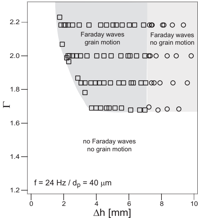
FIG. 9. Phase diagram in the parameters plane \Gamma - \Delta h , for f = 24 Hz and d_p = 40\mu m .
