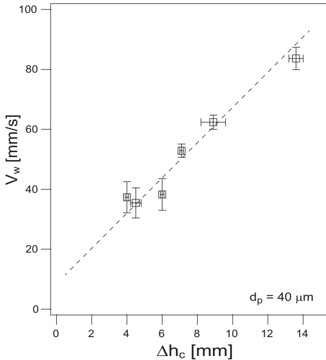
FIG. 11. Experimental relation between the depth of the supernatant liquid at the onset of grains motion, \Delta h_c , and the velocity scale based on the wave height, V_w = h_w f/2 .
