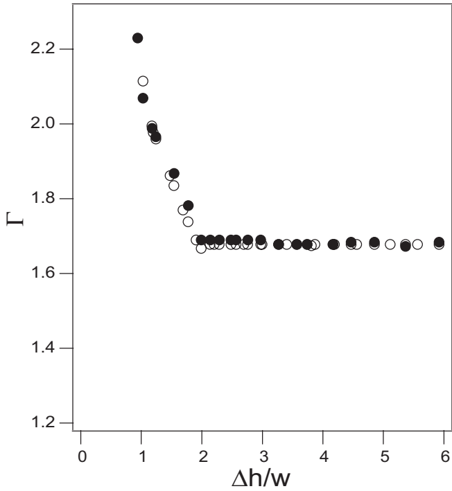
FIG. 2. Threshold of Faraday instability as a function of the reduced acceleration, \Gamma , and supernatant liquid depth, \Delta h , for f = 24 \text{ Hz} . Empty circles: only fluid. Filled circles: fluid plus particles.
