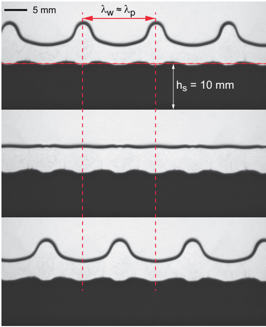
FIG. 6. Bed profiles at the Faraday threshold for f = 24 \text{ Hz} and \Delta h/w = 2.5 .
