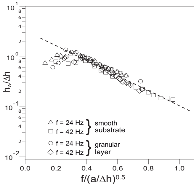
FIG. 4. The dimensionless wave height, h_w/\Delta h , as a function of f/\sqrt{a/\Delta h} , for measurements above the layer of motionless grains and the acrylic bottom of the cell. Equation 1 is plotted in black dashed line for fitting coefficients \alpha = 1.21 and \beta = 0.51 .
