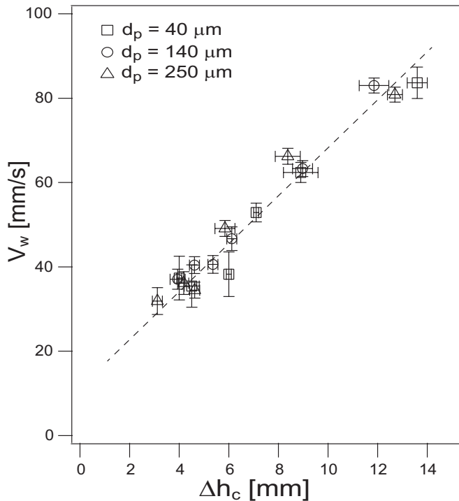
FIG. 13. Wave based velocity scale, V_w = h_w f / 2 , against the critical depth of the supernatant fluid, \Delta h_c , for different grain diameters, d_p .
