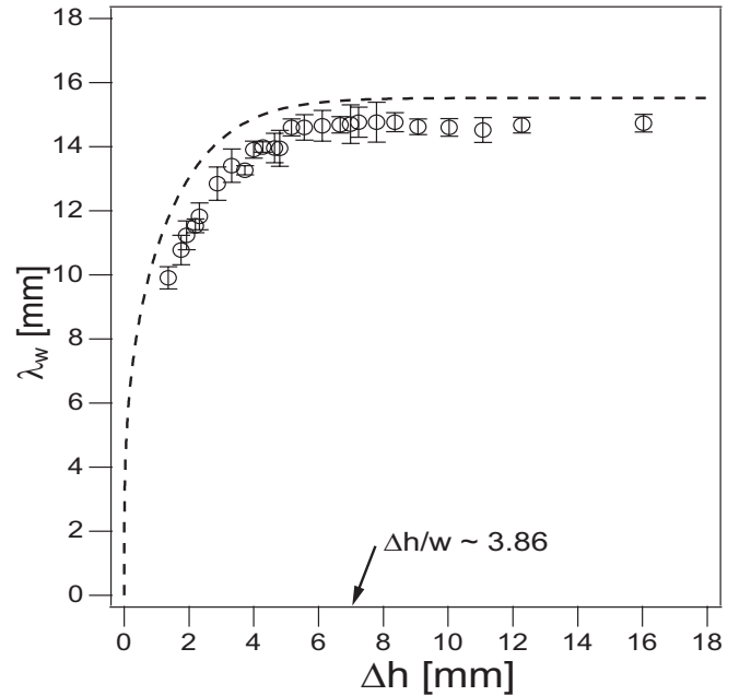
FIG. 5. Wavelengths of the Faraday waves as a function of \Delta h at the onset of Faraday instability for f = 24 Hz. Dashed line corresponds to the theoretical wavelength from the dispersion relation, Eq. 2, for a nonviscous fluid in an unbounded domain.
