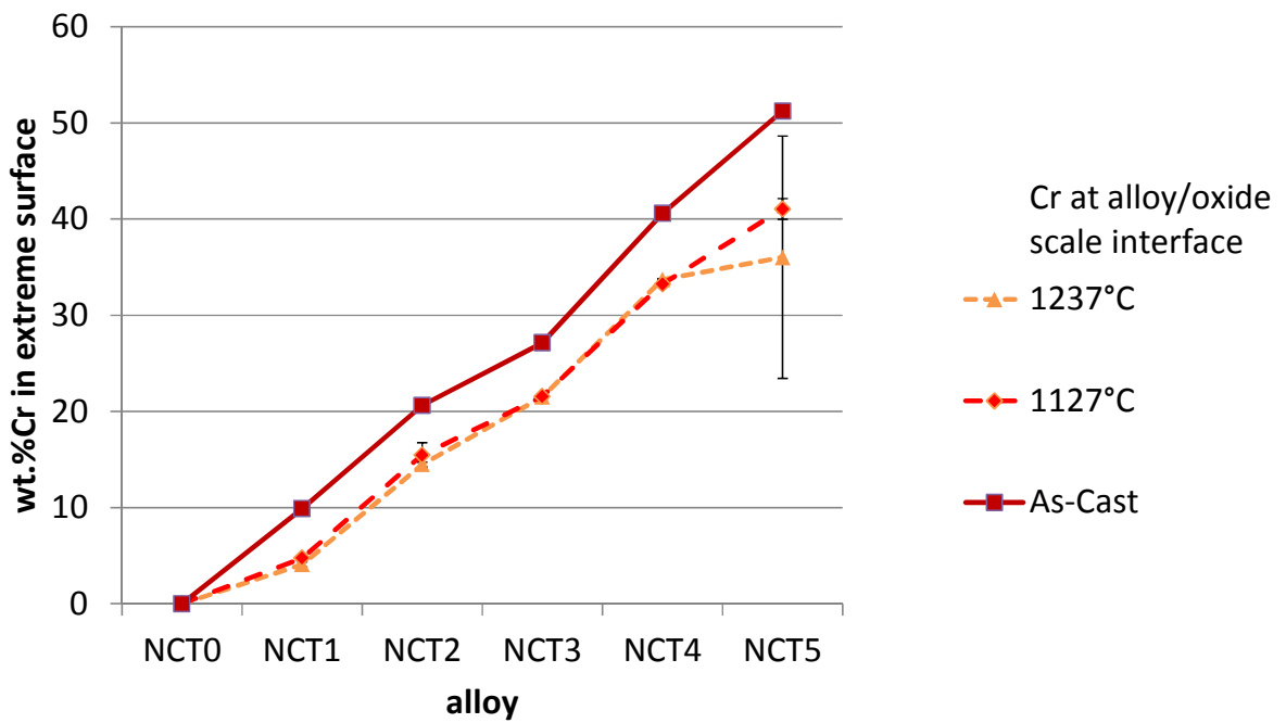
FIGURE 14. Chromium weight content in the subsurface very close to the oxidation front for the six alloys after 24 h at 1127°C and at 1237°C in laboratory air
