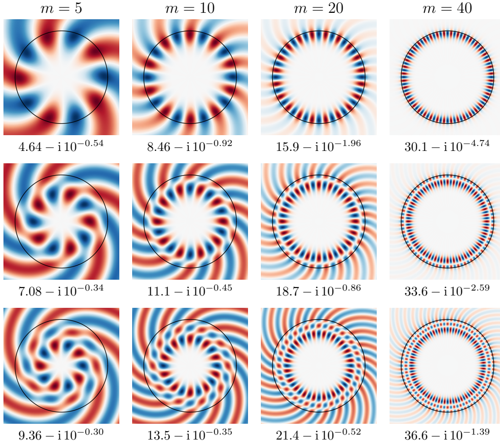
FIGURE 2. Plots of real parts of TM modes u in a circular cavity of radius R = 1 and index n = 1.5 (computed by solving the modal equation (1.4) using complex integration [22]). Below each plot, we give values of computed resonances k \in \mathbb{C} . Each row corresponds to a distinct value of j , from 0 to 2.
