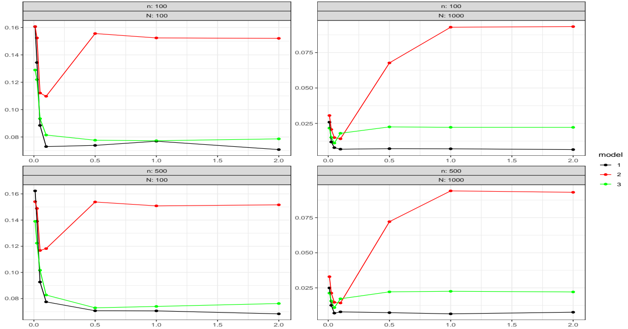
Figure 1: For models 1, 2, 3 estimates of the empirical risk \|\hat{b}_{\hat{K}} - \tilde{b}\|_{n,b}^2 for the chosen estimator \hat{b}_{\hat{K}}(c) = \hat{b}_{\hat{K}} as a function of c \in \mathcal{C} = \{0.01, 0.025, 0.05, 0.1, 0.5, 1, 2\}
