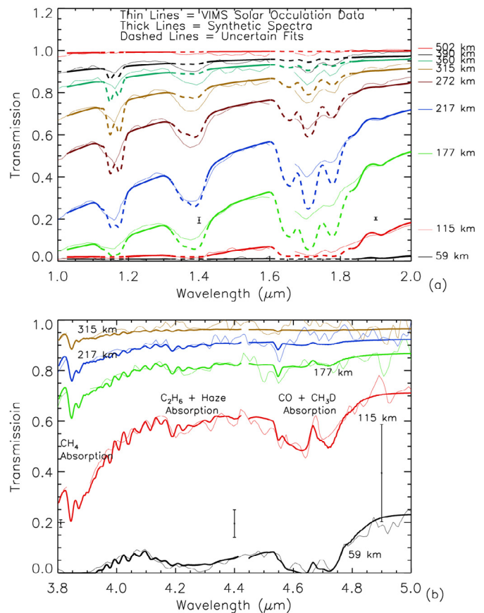
Fig. 1. Comparison between synthetic spectra and the VIMS spectra. a) In the 1–2 \mu\text{m} range for the selected altitudes of 59, 115, 177, 217, and 315 km. Wavelength intervals in which the model fits are not satisfactory are shown by dashed lines; they correspond to the centers of the \Delta\nu = 3, 4, and 5 bands of \text{CH}_4 near 1.7, 1.4, and 1.2 \mu\text{m} . b) In the 3.8–5 \mu\text{m} range at the selected altitudes of 59, 115, 177, 217, and 315 km. The synthetic spectra include the influence of \text{CH}_4 , \text{CH}_3\text{D} , \text{C}_2\text{H}_6 , \text{CO}_2 , CO, and haze absorption and scattering. The \pm 2\sigma error bars for the 1–1.6, 1.8–2, 3.8–4.8, and 4.8–5 \mu\text{m} intervals of the VIMS spectra are adopted from Bellucci et al. (2009).
