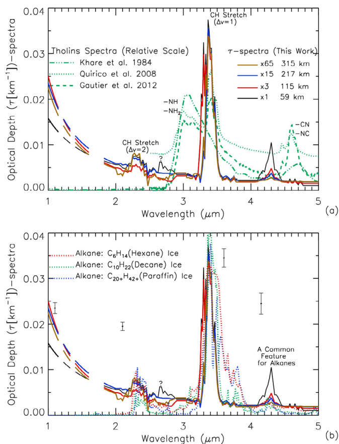
Fig. 2. Comparison between the derived haze \tau -spectra (at the selected altitudes of 59, 115, 217, and 315 km) and the spectra of a) tholins and b) alkane ices. Between 1 and 2 \mu\text{m} , we discarded the wavelength intervals (shown as dashed lines in Fig. 1a) in which the \tau -spectra are most uncertain. a) The tholin spectra are adopted from the literature (Khare et al. 1984; Quirico et al. 2008; Gautier et al. 2012). b) Spectra measured (Clark et al. 2009) for the alkane powders C 6 H 14 (hexane), C 10 H 22 (decane), and C 20+ H 42+ (paraffin) provide a satisfactory fit to the three major peaks of the haze \tau -spectra at 2.3, 3.4, and 4.3 \mu\text{m} . The \pm 1\sigma error bars for the 1–1.6, 1.8–3, 3–3.9, and 3.9–4.8 \mu\text{m} intervals of the \tau -spectra are shown.
