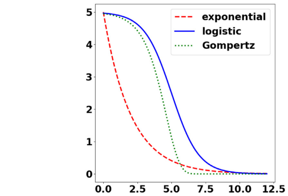
Fig. 19. Shape of several growth laws z \mapsto V(z) (x-axis: z , size of the tumor cells, y-axis: growth rate of the cells).
