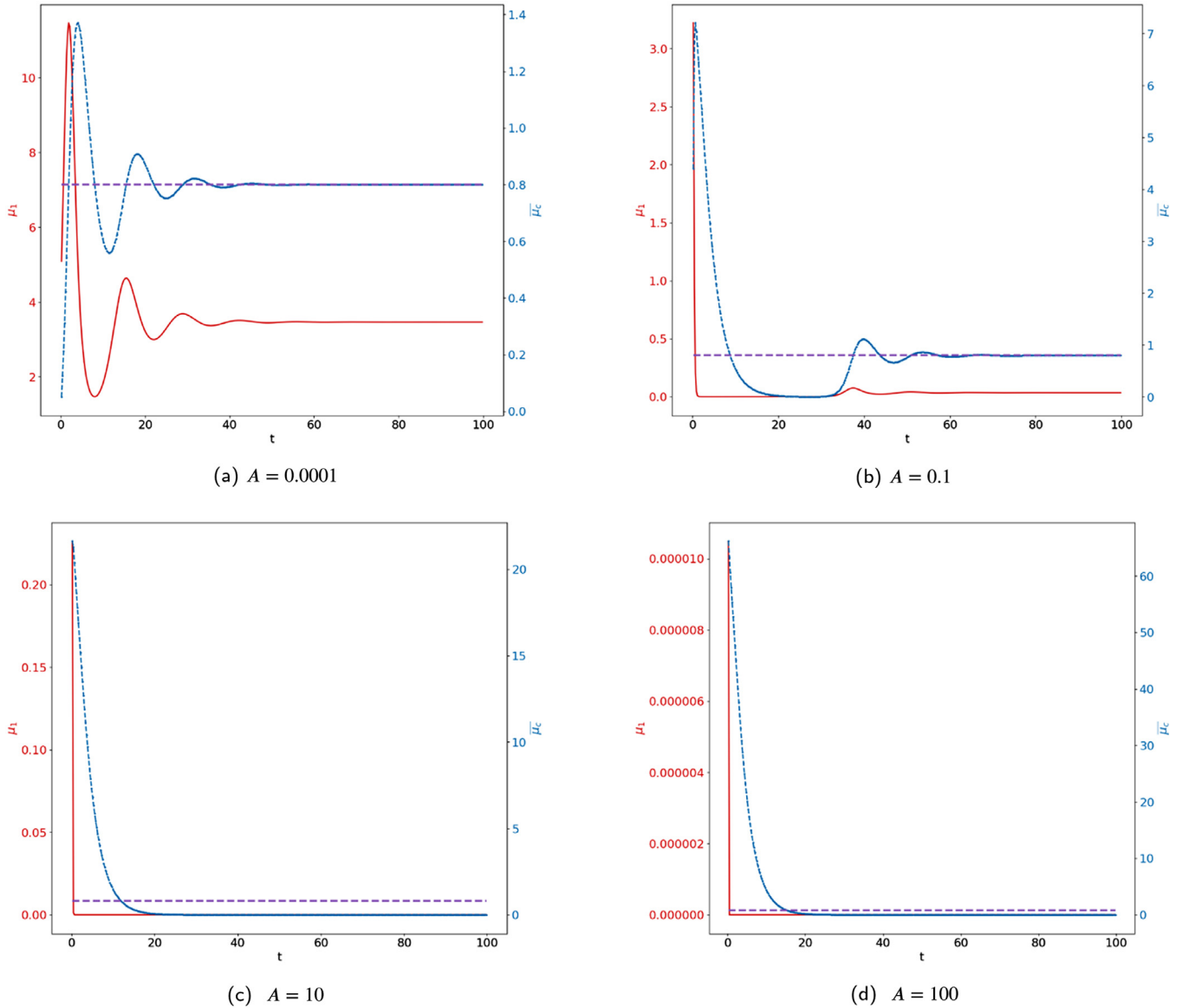
Fig. 9. Non saturated interactions, homogeneous source of immune cells. Evolution of the tumor mass \mu_1 (red curves, left axis), and of \bar{\mu}_c (blue curve, right axis) for several values of A .
