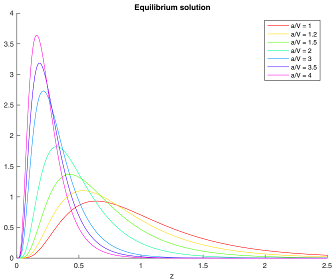
Fig. 3. Shape of the leading eigen-function of the growth-division equation for several values of \frac{a}{V} (x-axis: z, size of the tumor cells, y-axis: number of tumor cells at the final time).
