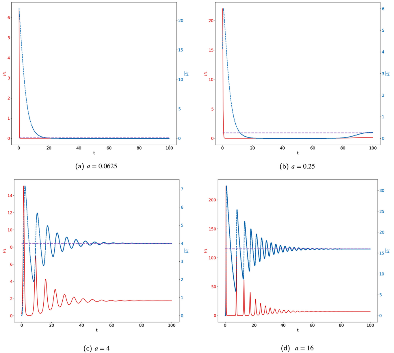
Fig. 7. Non saturated interactions, homogeneous source of immune cells. Evolution of the tumor mass \mu_1 (red curves, left axis), and of \bar{\mu}_c (blue curve, right axis) for several values of the division rate a .
