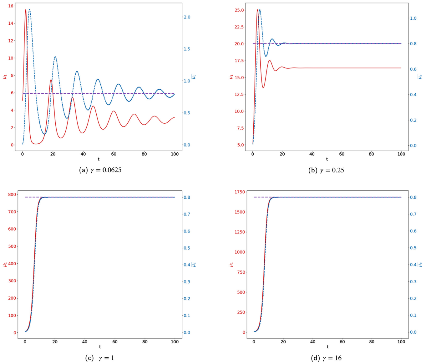
Fig. 15. Non saturated interactions, heterogeneous source of immune cells. Evolution of the tumor mass \mu_1 (red curves, left axis), and of \bar{\mu}_c (blue curve, right axis) for several values of the immune cells death rate \gamma .
