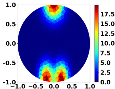
Fig. 12. Heterogeneous source of immune cells S (the axis correspond to the space coordinates).
