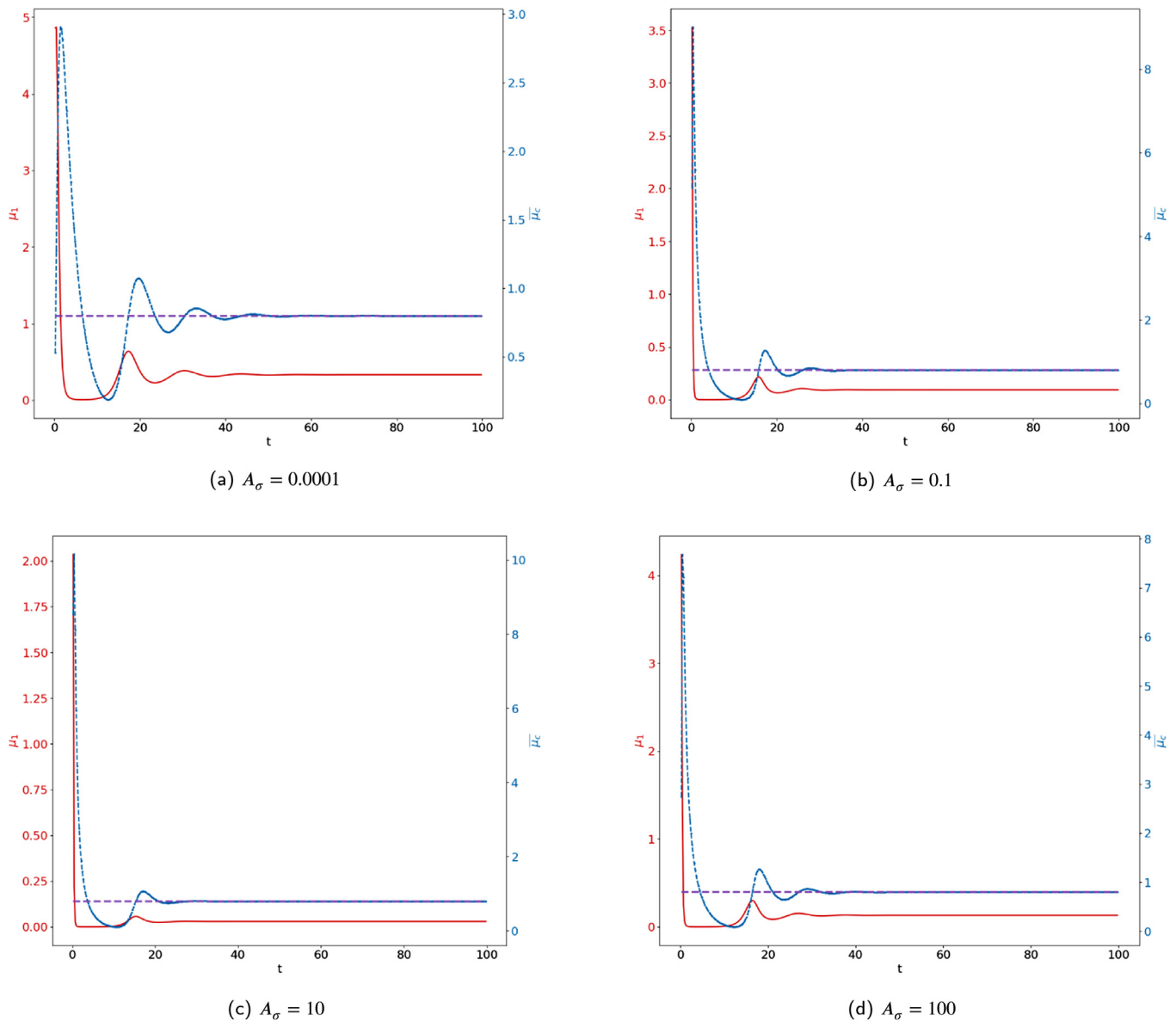
Fig. 10. Non saturated interactions, homogeneous source of immune cells. Evolution of the tumor mass \mu_1 (red curves, left axis), and of \bar{\mu}_c (blue curve, right axis) for several values of A_\sigma .
