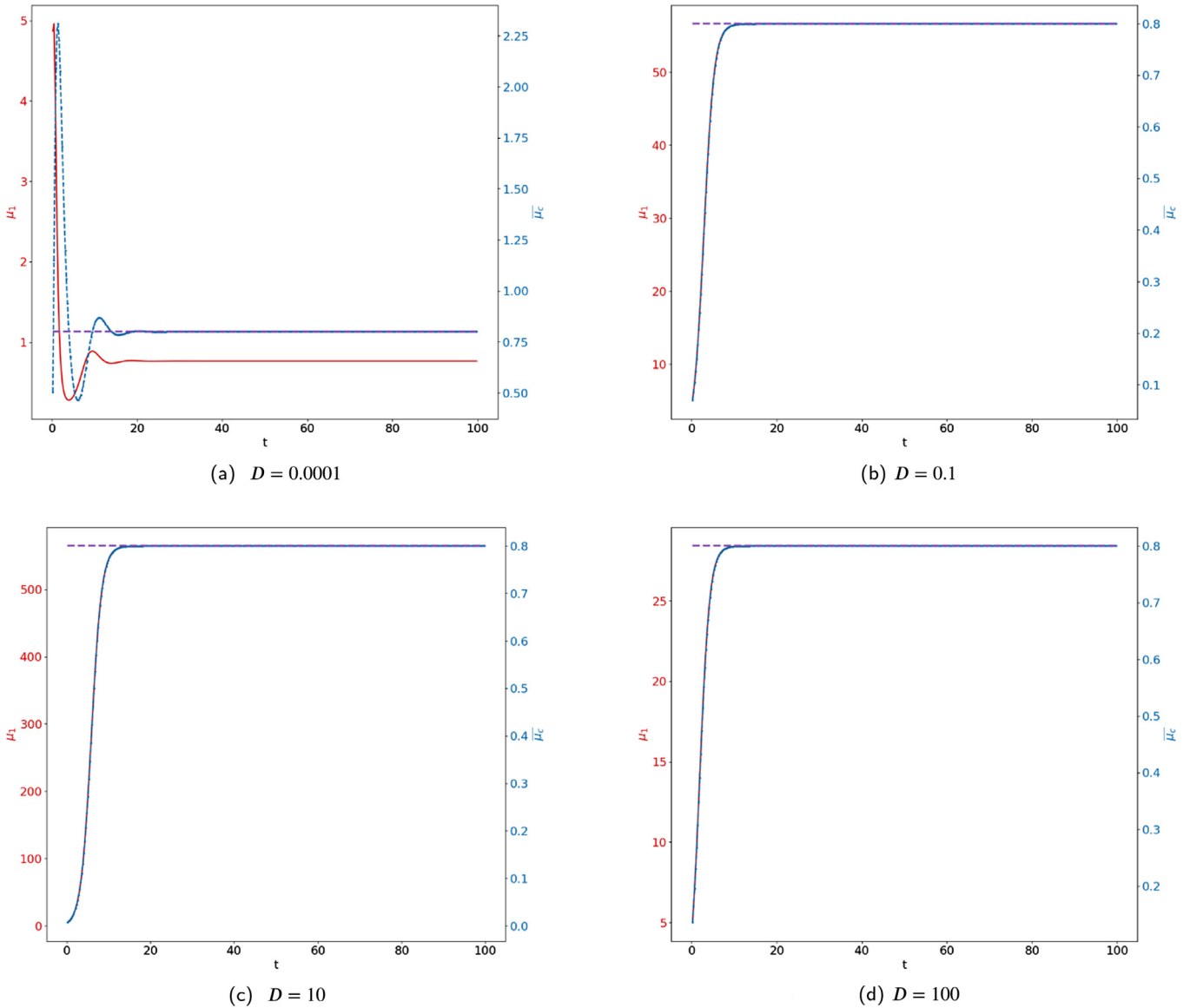
Fig. 11. Non saturated interactions, homogeneous source of immune cells. Evolution of the tumor mass \mu_1 (red curves, left axis), and of \bar{\mu}_c (blue curve, right axis) for several values of the diffusion coefficient D .
