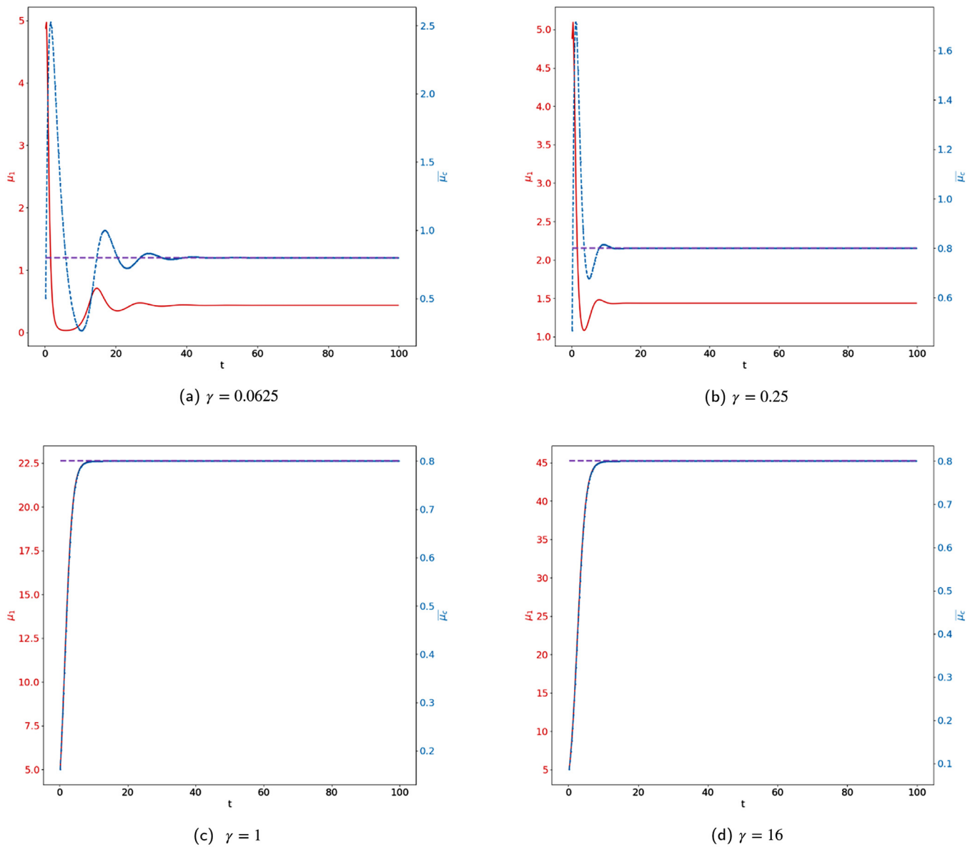
Fig. 8. Non saturated interactions, homogeneous source of immune cells. Evolution of the tumor mass \mu_1 (red curves, left axis), and of \bar{\mu}_c (blue curve, right axis) for several values of the immune cells death rate \gamma .
