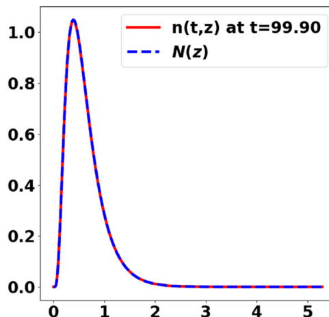
Fig. 4. Convergence to the asymptotic profile. Left: Time evolution of the tumor profile. Right: Comparison of the tumor size-distribution at T = 99.90 with the exact asymptotic state (x-axis: z, size of the tumor cells, y-axis: number of tumor cells at the final time).
