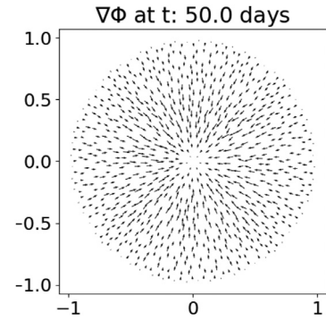
Fig. 5. Non saturated interactions, homogeneous source of immune cells: the gradient of the chemotactic potential at t = 50.0 (the axis correspond to the space coordinates).
