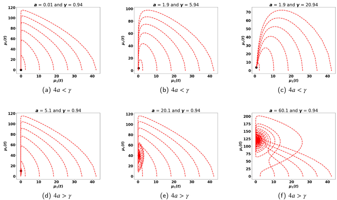
Fig. 2. Typical phase portraits ( \mu_1 , \mu_c ) of (25) for different initial tumor mass. The data are: V = 0.616 , \delta = 0.5 , p = 4.66 , S = 6.38 .
