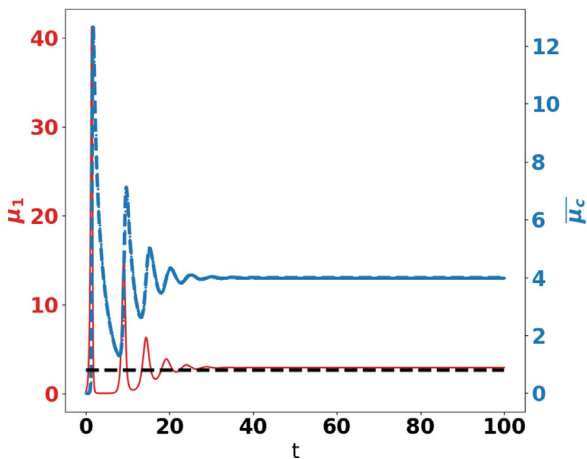
Fig. 18. Non saturated interactions, heterogeneous source of immune cells. Evolution of the tumor mass \mu_1 (red curves, left axis), and of \bar{\mu}_c (blue curve, right axis) with a = 4 and \chi = 100 .
