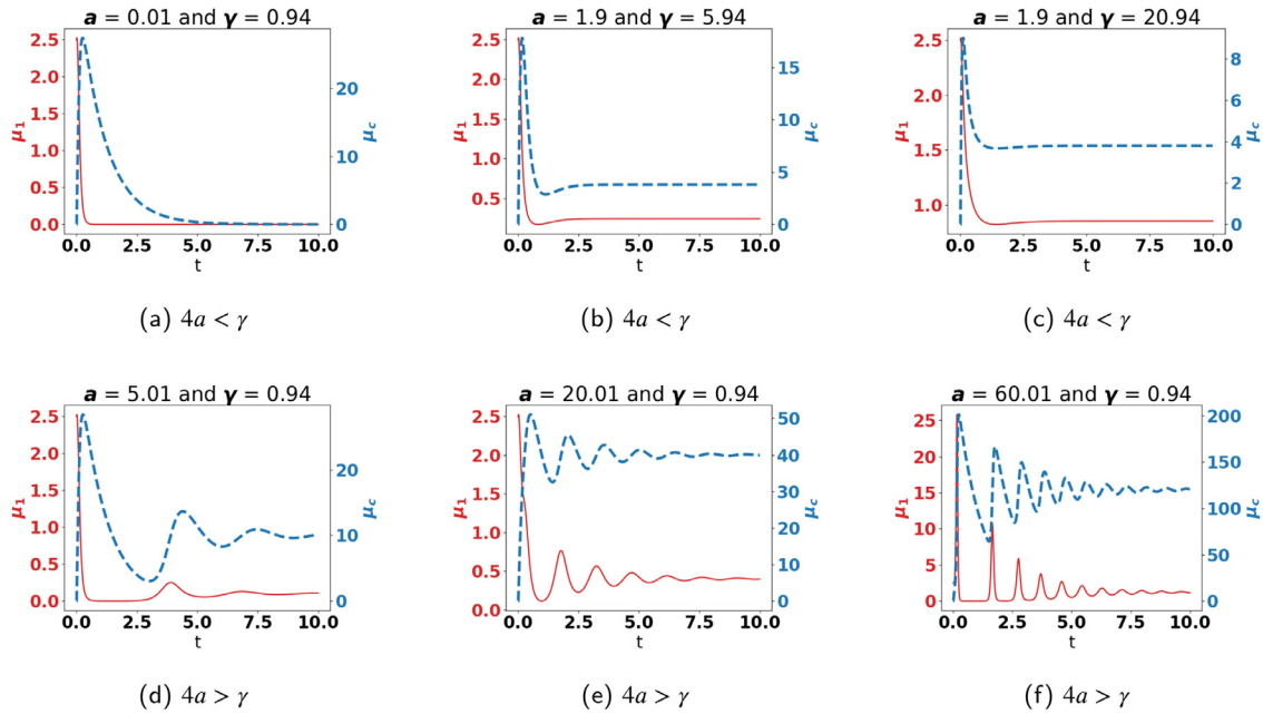
Fig. 1. Typical behavior of the solutions of (25). The data are: V = 0.616 , \delta = 0.5 , p = 4.66 , S = 6.38 (x-axis: time, y-axis: \mu_1 , mass of the tumor, and \mu_c , the total number of active immune cells).
