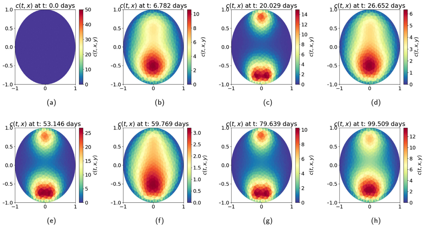
Fig. 13. Time evolution of the cytotoxic effector cells concentration c(t, x) (the axis correspond to the space coordinates).
