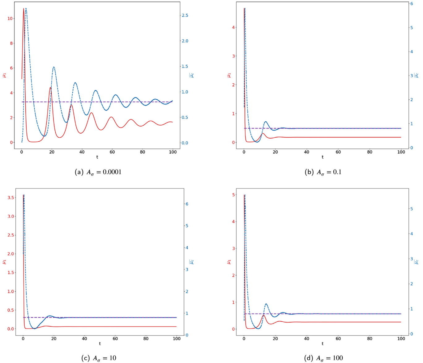
Fig. 17. Non saturated interactions, heterogeneous source of immune cells. Evolution of the tumor mass \mu_1 (red curves, left axis), and of \bar{\mu}_c (blue curve, right axis) for several values of A_\sigma .
