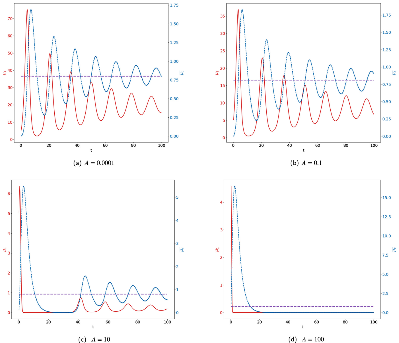
Fig. 16. Non saturated interactions, heterogeneous source of immune cells. Evolution of the tumor mass \mu_1 (red curves, left axis), and of \bar{\mu}_c (blue curve, right axis) for several values of A .
