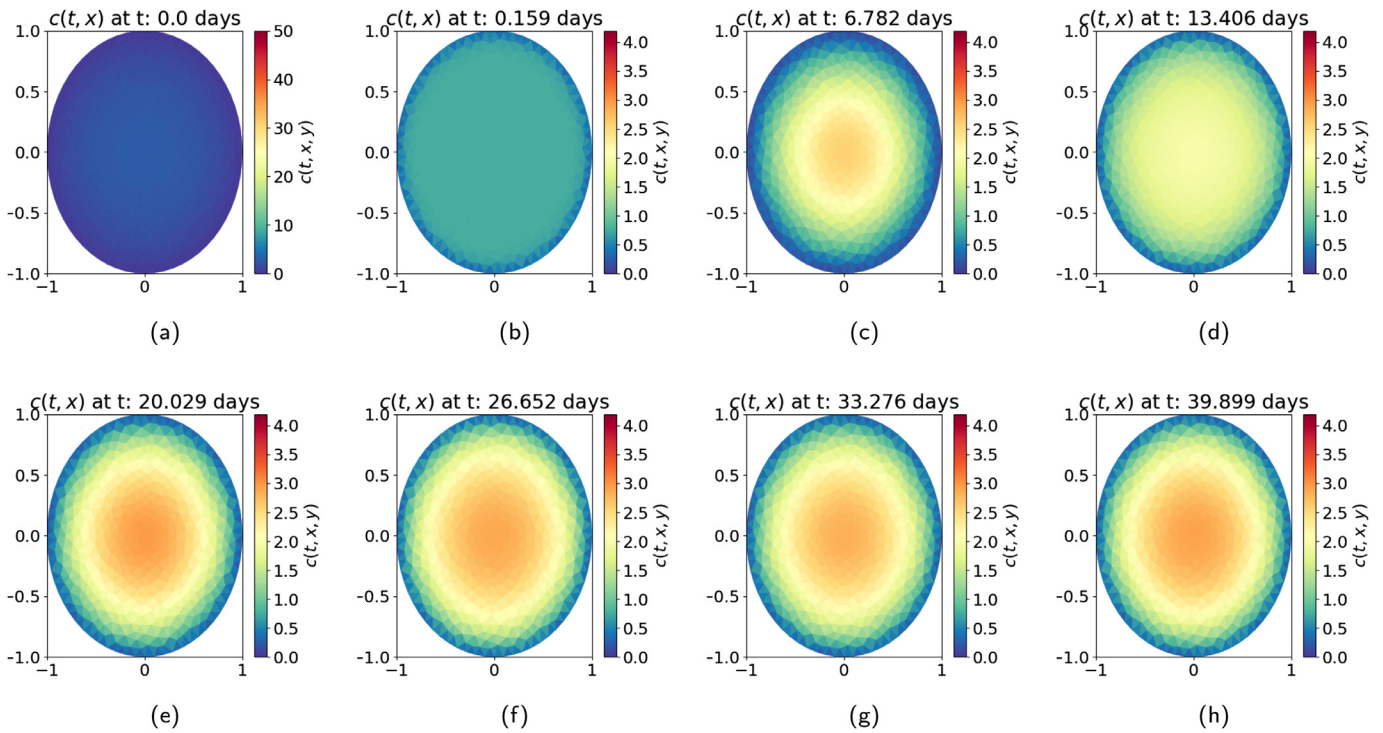
Fig. 6. Non saturated interactions, homogeneous source of immune cells: time evolution of the cytotoxic effector cells concentration c (the axis correspond to the space coordinates).
