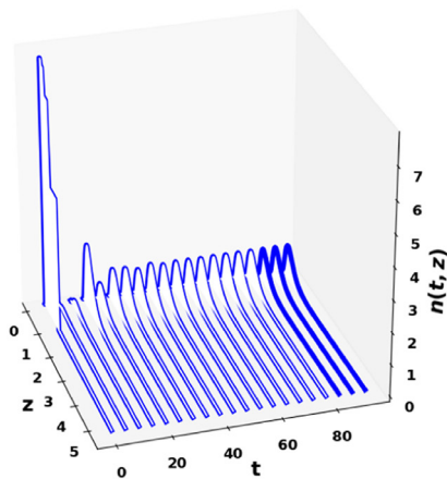
Fig. 4. Convergence to the asymptotic profile. Left: Time evolution of the tumor profile. Right: Comparison of the tumor size-distribution at T = 99.90 with the exact asymptotic state (x-axis: z, size of the tumor cells, y-axis: number of tumor cells at the final time).
