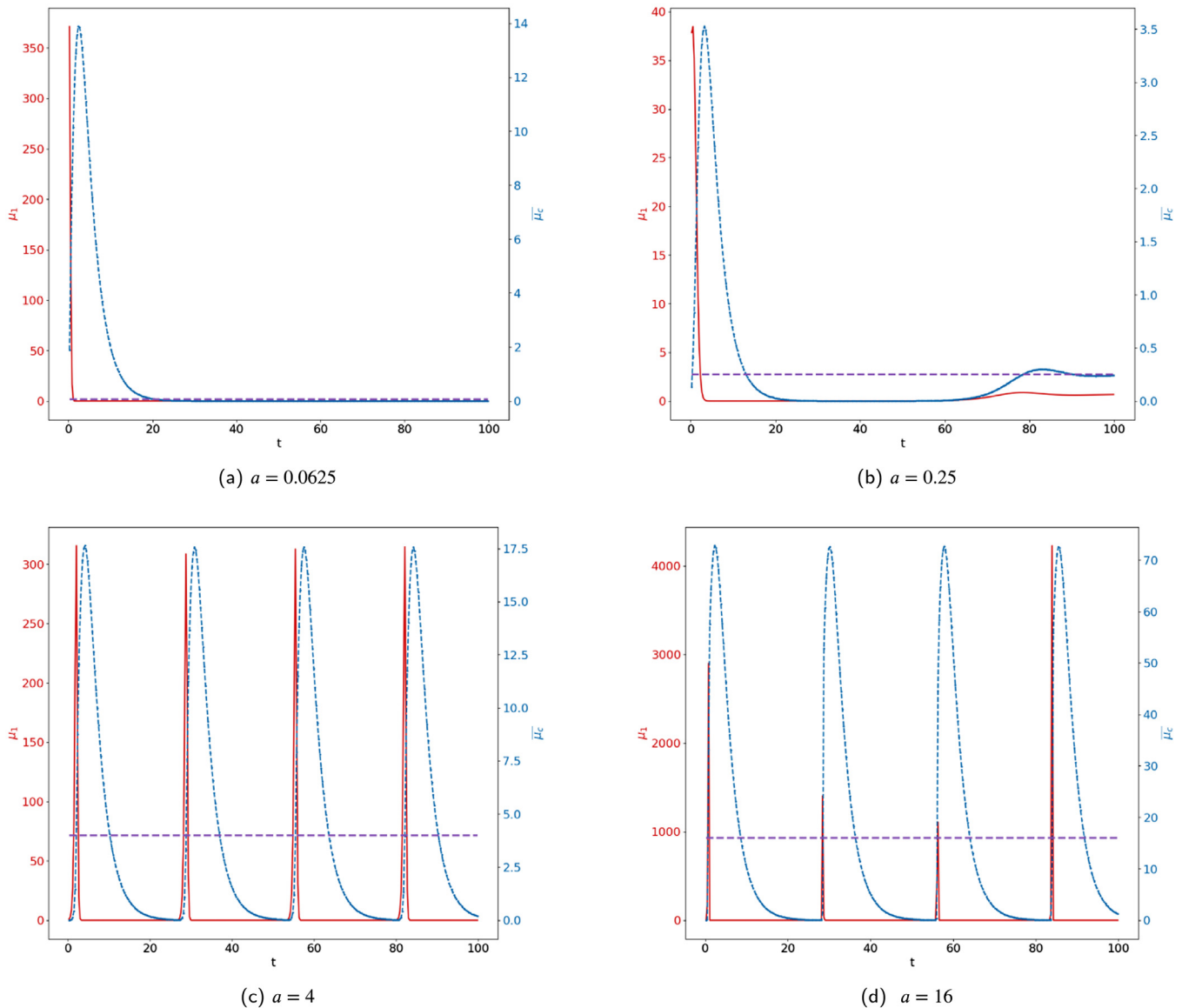
Fig. 14. Non saturated interactions, heterogeneous source of immune cells. Evolution of the tumor mass \mu_1 (red curves, left axis), and of \bar{\mu}_c (blue curve, right axis) for several values of the division rate a .
