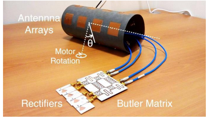
Fig. 4. (a) Scheme and (b) experimental prototype of the multi-directional RF energy harvester composed of passive beam-forming networks [15].
