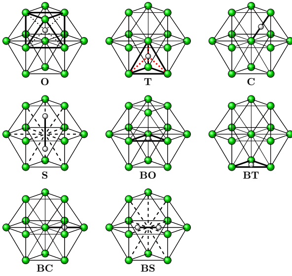
Figure 2: Eight interstitial configurations in hcp beryllium
