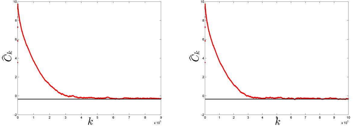
Figure 10: Evolution of \widehat{C}_k in Algorithm 1 when applied to \mathcal{X}_{mN} = \mathcal{X}_N \cup \mathcal{X}_N^{(2)} \cup \dots \cup \mathcal{X}_N^{(m)} , the horizontal black line corresponds to C_{1-\alpha}(\mathbf{M}_\alpha^*) . Left: n = 100 , N = 100\,000 , m = 9 ; Right: n = 1\,000 , N = 1\,000\,000 , m = 1 .
