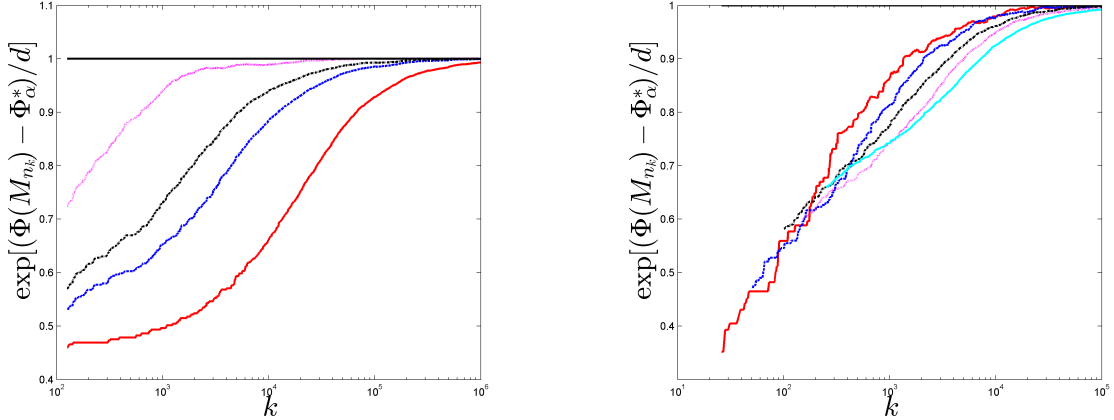
Figure 6: Evolution of D-efficiency of \mathbf{M}_{n_k} obtained with Algorithm 1 as a function of k (log scale); the horizontal line indicates the optimal value 1. Left: d = 25 and \alpha = 0.5 (magenta dotted line), 0.1 (black), 0.05 (blue) and 0.01 (red solid line). Right: \alpha = 0.1 and d = 5 (red solid line), 10 (blue), 20 (black), 30 (magenta) and 50 (cyan solid line).
