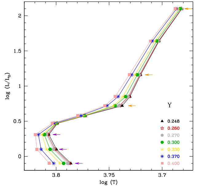
Fig. 1. Hertzsprung-Russell diagram (HRD) showing isochrones computed by Chantreau et al. (2015) for a metallicity of [Fe/H] = -1.53 . Different colors correspond to different chemical compositions, labeled by their initial helium mass fraction. Symbols correspond to positions along the isochrones where atmosphere models and synthetic spectra have been calculated. The arrows indicate the models used for binary combinations.
