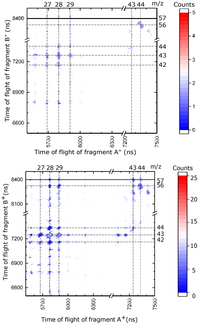
Fig. 11 Map of the correlation between A^+ and B^+ fragments, corresponding to the fragmentation of the hydantoin dication after collision with \text{He}^{2+} at 8 keV (a) and \text{O}^{6+} at 30 keV (b).
