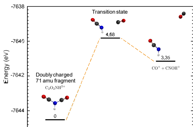
Fig. 13 Calculated fragmentation path from 71^{2+} to 28^{+} + 43^{+} . Energies levels are in eV and referenced against 71^{2+} optimized geometry.
