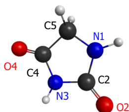
Fig. 1 Neutral form of Hydantoin in the ground state (labels from 27 ).
