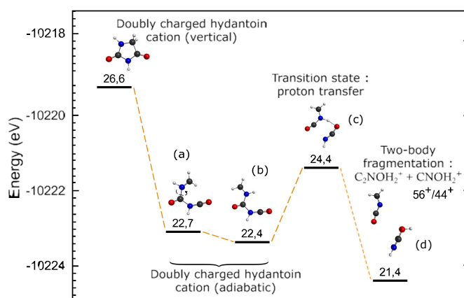
Fig. 15 Calculated fragmentation path corresponding to the two body \text{Hyd}^{2+} to 44^{+} + 56^{+} . Energies levels are in eV and referenced against neutral hydantoin optimized geometry.
