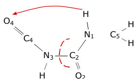
Fig. 16 Two body fragmentation \text{Hyd}^{2+}(100^{2+}) \rightarrow 56^+ + 44^+ , via a proton transfer.
