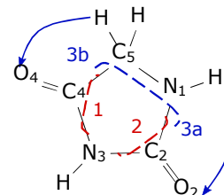
Fig. 6 Formation of m/z=72 fragment via the loss of neutral CO (1 and 2) or neutral CNH_2 (3a and 3b).
