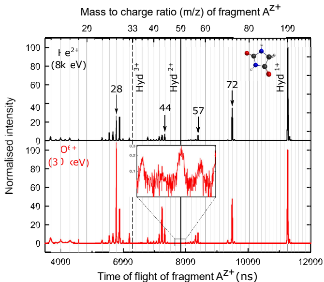
Fig. 5 Inclusive mass spectra of cations arising from the fragmentation of neutral hydantoin molecule C_3N_2O_2H_4 after collision with He^{2+} at 8 keV and O^{6+} at 30 keV. The inset is a zoom on the m/z=50 peak structure, corresponding to the unfragmented Hyd^{2+} parent ion (intensity is in log scale).
