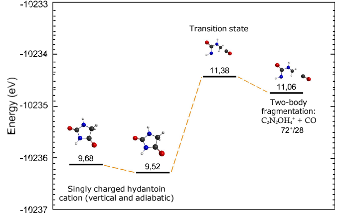
Fig. 8 Calculated two body fragmentation path leading to the formation of 72 amu cation via the loss of neutral \text{C}^{(4)}\text{O}^{(4)} . Energies levels are referenced against the neutral hydantoin molecule.
