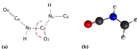
Fig. 14 (a) Localisation of the 57 amu fragment on the hydantoin molecule dication (b) Optimized geometry (numerical calculation) of the 57^{2+} fragment.
