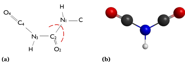
Fig. 12 (a) Localisation of the 71 amu fragment on the hydantoin molecule dication (b) Optimized geometry (numerical calculation) of the 71^{2+} fragment.
