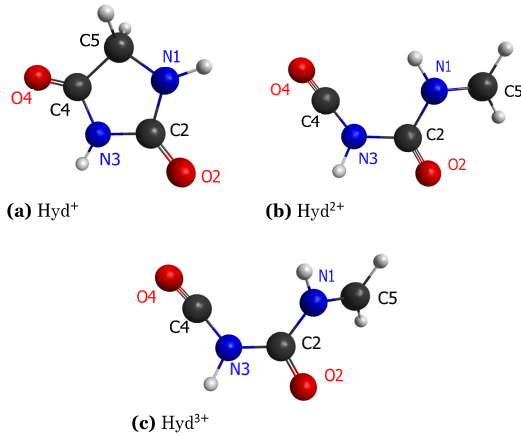
Fig. 3 Hydantoin relaxed geometries for the different charge states of the molecule.
