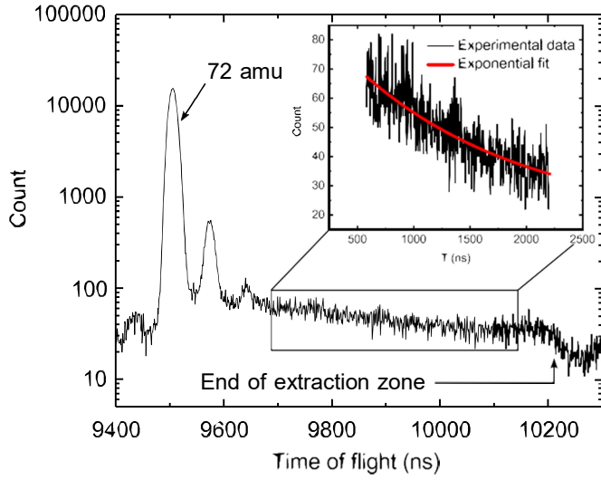
Fig. 7 Intensity distribution on the mass range around m/z = 72 for \text{He}^{2+} projectile. The inset correspond to the delayed tail, fitted by an exponential. In this zoom, the time on abscissa axis is the delayed fragmentation time of the hydantoin molecule.
