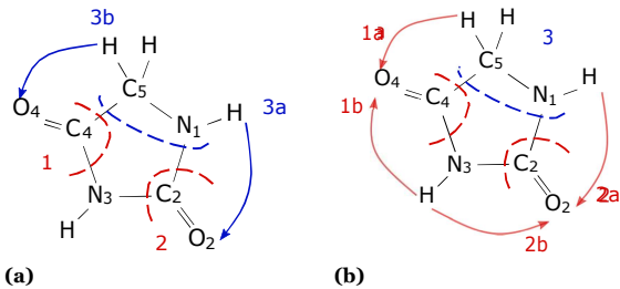
Fig. 9 Location of fragment m/q=28 (a) and fragment m/q=29 (b) coming from \text{Hyd}^{1+} cation.
