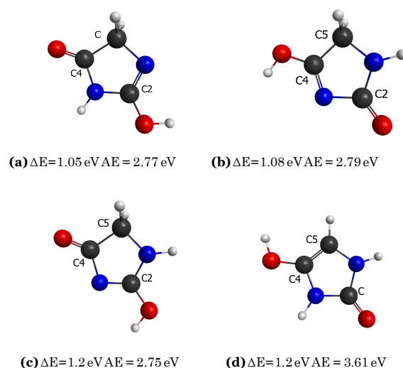
Fig. 2 Calculated geometries and energies of the tautomer form of the neutral hydantoin molecule. AE = activation barrier, \Delta E = adiabatic energy.
