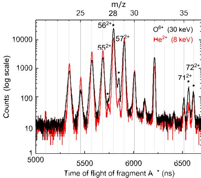
Fig. 10 Zoom on the inclusive spectra arising from the fragmentation of charged hydantoin molecule after collision with \text{He}^{2+} at 8 keV and \text{O}^{6+} at 30 keV. Peaks corresponding to doubly charged fragments are labelled by stars.
