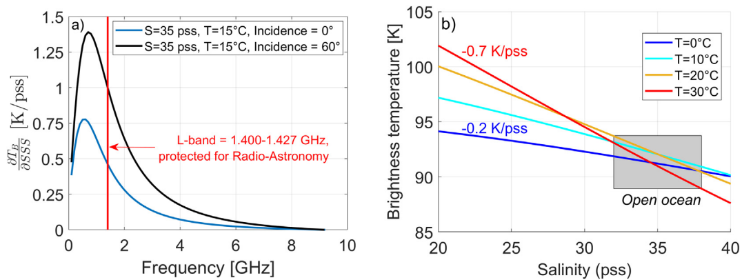
Fig. 3. (a) sensitivity of the ocean surface microwave brightness temperature to Salinity (First Stokes parameter) as a function of electromagnetic frequency and incidence angle (blue curve = 0^\circ , black curve = 60^\circ ) and for a water body with salinity of 35 pss and temperature of 15^\circ\text{C} . (b) Brightness temperature ((T_H + T_V)/2) changes at 1.4 GHz and nadir as a function of salinity (x-axis) and temperature (colors). The gray domain indicates the range of SSS values mostly encountered in the open ocean. (For interpretation of the references to color in this figure legend, the reader is referred to the web version of this article.)
