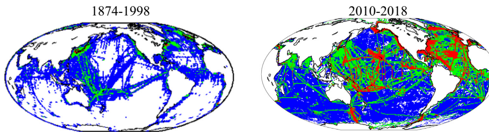
Fig. 1. (Left) Number of historical in situ SSS observations over 125 years from 1874 to 1998 per 1^\circ square (from Bingham et al., 2002). Note that only few WOCE lines were available into the NODC database used to build the density map (personal exchanges with F. Bingham). (Right) Number of historical in situ SSS observations per 1^\circ square during the first 9 years of the satellite salinity era from 2010 to 2018. Blue, > 10 observations; green, > 100 observations; and red, > 1000 observations. No color means < 10 observations. (For interpretation of the references to color in this figure legend, the reader is referred to the web version of this article.)
