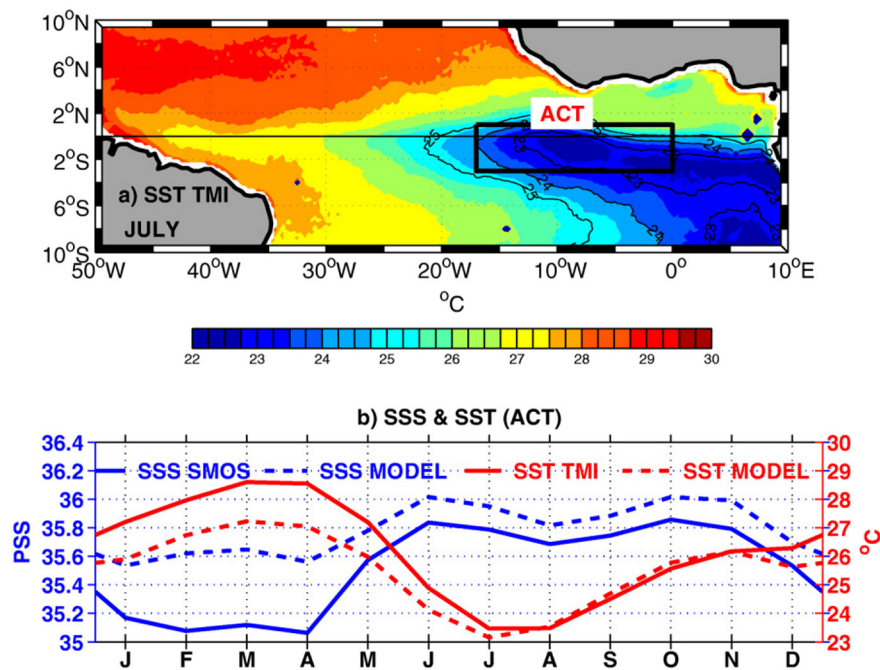
Fig. 25. (a) Averaged map of the microwave (TMI) SST [ ^{\circ} C] in July in the equatorial Atlantic. Contour levels are at 23, 24, and 25 ^{\circ} C. The black contoured box indicate the equatorial Atlantic Cold tongue (ACT) study area. (b) Seasonal change of SSS (blue curves) and SST (red curves) in the ACT region averaged over 2010–2012. Satellite data (solid); Model data (dashed). From Da-Allada et al., 2017. (For interpretation of the references to color in this figure legend, the reader is referred to the web version of this article.)
