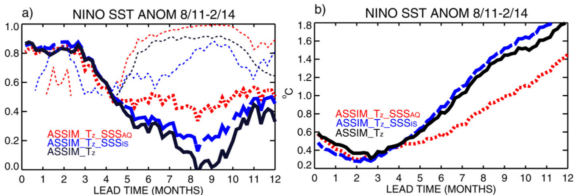
Fig. 18. (a) Correlation coefficient and (b) RMS difference of the model SST forecasts with the observed NiNO3 SST anomaly. The period considered is August 2011 to February 2014. The solid black curve is initialized using assimilation of subsurface temperature (ASSIM_Tz), the thick dotted red curve from subsurface temperature and Aquarius SSS (ASSIM_Tz_SSSAQ) and the dash blue curve from subsurface temperature and weekly OI of all available near-surface salinity (ASSIM_Tz_SSSIS). The thin dotted curves indicate the corresponding significance of the differences from a Fisher Z test. After Hackert et al. (2014). (For interpretation of the references to color in this figure legend, the reader is referred to the web version of this article.)
