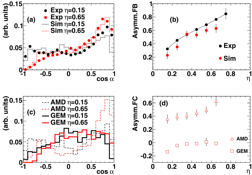
FIG. 8. (a) \cos \alpha distribution for two different windows of \eta , experimental data (symbols) and AMD+GEMINI simulation (histograms). (b) Asymm.FB vs. \eta , experimental (black symbols) and simulated (red symbols) data. (c) \cos \alpha distribution for two different windows of \eta , simulated data. Full histograms: fissions performed by GEMINI. Dash-dotted histograms: fissions performed by AMD. (d) Asymm.FC vs. \eta , simulated data. Open squares: fissions performed by GEMINI. Open triangles: fissions performed by AMD. In (a) and (c) the spectra are scaled in order to have total integral equal to 1.
