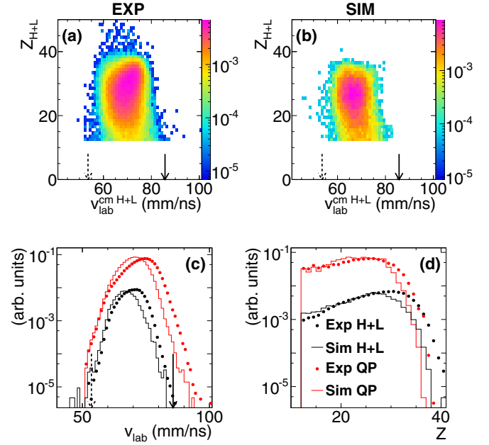
FIG. 4. Top: Z_{H+L} vs. laboratory velocity of the c.m. of the pair of fission fragments for the reaction ^{80}\text{Kr} + ^{48}\text{Ca} at 35 MeV/nucleon. (a) Experimental data. (b) Filtered simulated data (AMD with asystiff symmetry energy, followed by GEMINI++ as afterburner). Dashed arrow: c.m. velocity. Continuous arrow: beam velocity. Bottom: (c) Black symbols and histograms: laboratory velocity of the c.m. of the pair of fission fragments, experimental and simulated data; red symbols and histograms: laboratory velocity of the biggest fragment of the QP selection (d) black symbols and histograms: Z_{H+L} distribution, experimental and simulated data; red symbols and histograms: charge distribution of the biggest fragment of the QP selection. All the plots are scaled in such a way that the total integral is 1, except for the black symbols and curves of panels (c) and (d), where the ratio with respect to the QP curves is kept.
