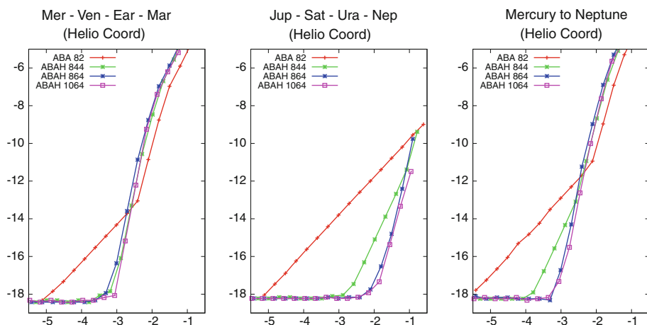
Fig. 6 Comparison between ABA\mathcal{H} schemes of order (8, 4, 4) , (8, 6, 4) and (10, 6, 4) specific for heliocentric coordinates and the ABA82 . From left to right the 4 inner planets, the 4 outer planets and the whole Solar System. The x -axis represents the cost (\tau/n) and the y -axis the maximum energy variation for one integration at constant step-size \tau (decimal log scales)
