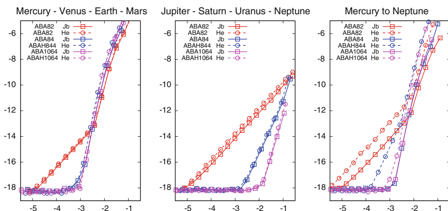
Fig. 7 Comparison between Jacobi ( continuous lines ) and heliocentric ( discontinuous lines ) coordinates using the schemes of orders (8, 2) (red), (8, 4) (blue) and (10, 6, 4) (purple). From left to right the 4 inner planets, the 4 outer planets and the whole Solar System. The x -axis represents the cost (\tau/s) of the method and the y -axis the maximum energy variation for one integration with constant step-size \tau (decimal log scales)
