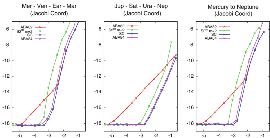
Fig. 2 Comparison between the different schemes to kill the \varepsilon^2\tau^2 terms in the ABA82 scheme. From left to right the 4 inner planets, the 4 outer planets and the whole Solar System. The x -axis represents the cost ( \tau/s ) and the y -axis the maximum energy variation for one integration with constant step-size \tau (decimal log scales)
