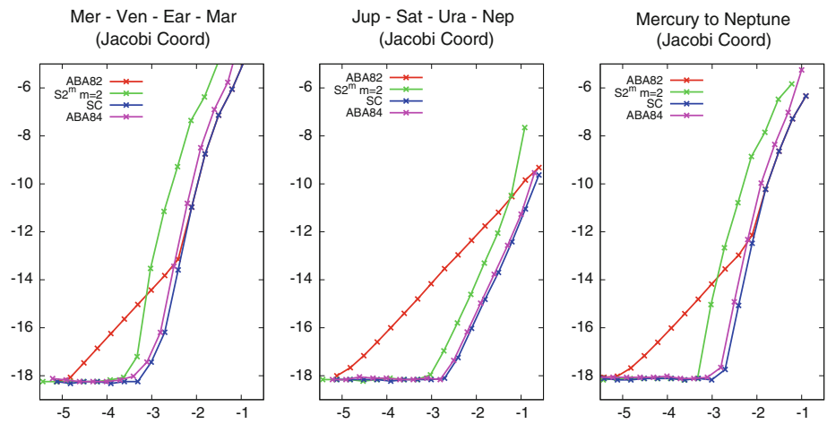
Fig. 2 Comparison between the different schemes to kill the \epsilon^2\tau^2 terms in the ABA82 scheme. From left to right the 4 inner planets, the 4 outer planets and the whole Solar System. The x -axis represents the cost ( \tau/s ) and the y -axis the maximum energy variation for one integration with constant step-size \tau (decimal log scales)
