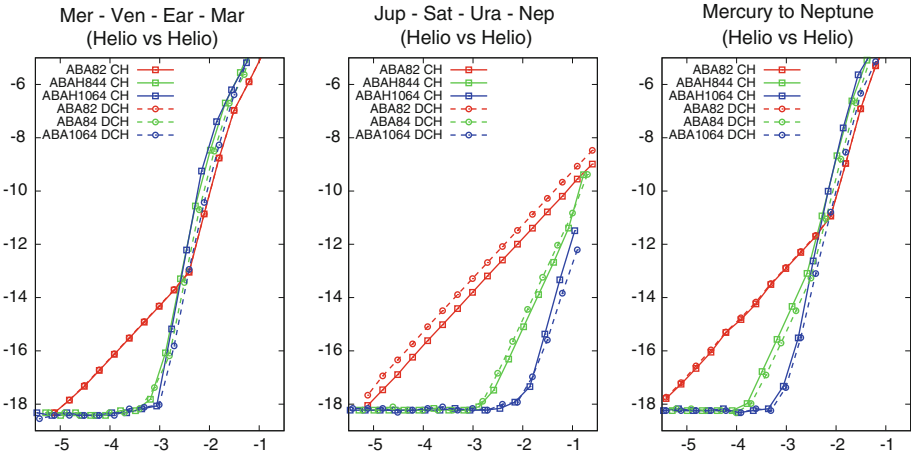
Fig. 9 Comparison between the two expressions for heliocentric coordinates: the classical CH expressions (Eqs. 44–46) continuous lines and the DCH expressions (Eqs. 47–49) discontinuous lines . For the schemes ABA82 (red), ABA84 (green) and ABA1064 (blue). From left to right the 4 inner planets, the 4 outer planets and the whole Solar System. The x -axis represents the cost ( \tau/s ) of the method and the y -axis the maximum energy variation for one integration with constant step-size \tau (decimal log scales)
