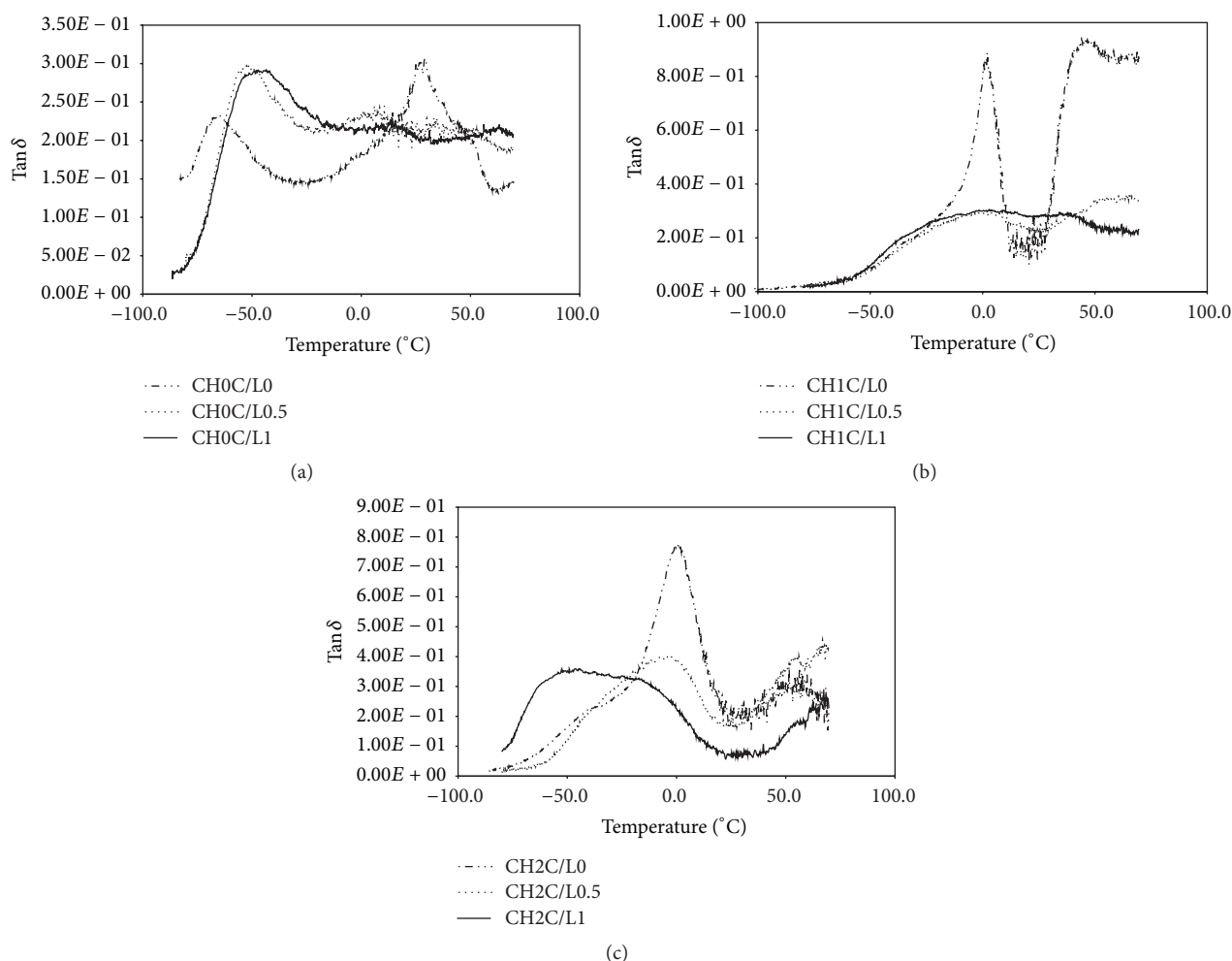
FIGURE 2: \tan \delta of HPMC, CH, and C/L preparation films of (a) CH0C/L0, CH0C/L0.5, and CH0C/L1; (b) CH1C/L0, CH1C/L0.5, and CH1C/L1; and (c) CH2C/L0, CH2C/L0.5, and CH2C/L1 variants.
