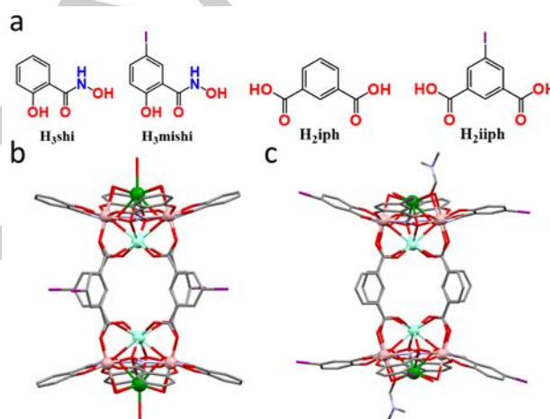
Figure 1. (a) Structural formulas of the hydroxamic acids ( \text{H}_3\text{shi} , \text{H}_3\text{mishi} ) and the bridging ligands ( \text{H}_2\text{iph} , \text{H}_2\text{iiph} ). Crystallographic structures of (b) Sm-I 4 and (c) Sm-I 8 . Sm: cyan; Ga: rose; O: red; N: light blue; C: grey; I: purple; Na: green. The hydrogen atoms and solvent molecules have been omitted for clarity.
