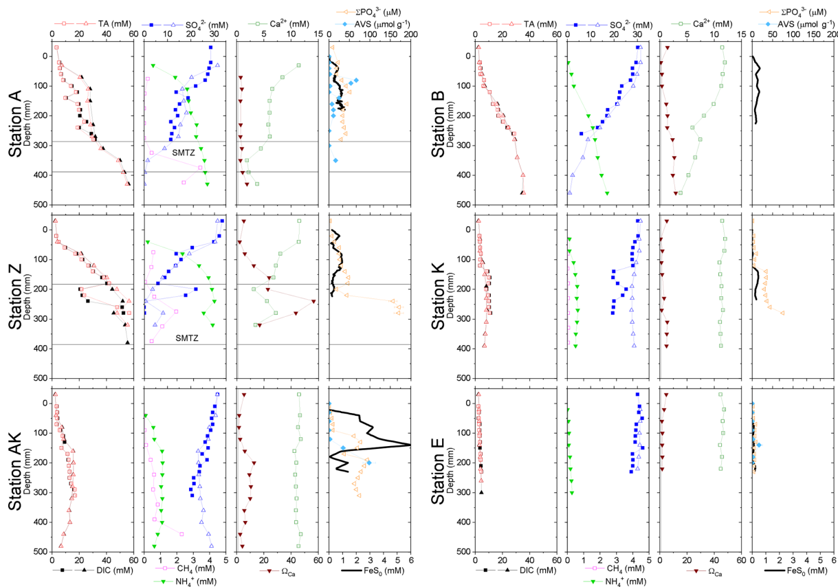
Figure 5. Depth profiles of pore water TA, DIC, SO_4^{2-} , NH_4^+ , CH_4 , Ca^{2+} , nanoparticulate FeS ( FeS_0 ), \Sigma PO_4^{3-} and AVS concentrations, along with the calcium carbonate (calcite) saturation state of the pore waters ( \Omega_{Ca} ) at stations A, Z, AK, K, B and E. Alternating symbol shapes indicate data collected from duplicate long and short sediment cores. The calcium carbonate (calcite) saturation state ( \Omega_{Ca} ) and pore water FeS_0 concentrations were calculated, whereas AVS was determined from solid-phase extractions. The two horizontal lines identify the sulfate–methane transition zone (SMTZ) found at stations A and Z. Error bars represent standard deviations of multiple measurements for the concentrations and error propagation for \Omega . Concentrations of CH_4 were not measured at stations B, K and E.
