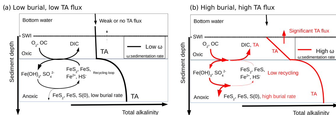
Figure 8. Conceptual model for visualizing the link between the burial of iron sulfide minerals and benthic alkalinity fluxes in the case of low sedimentation and OC flux (black) and high sedimentation rates and OC flux (red). The total alkalinity (TA) produced under anaerobic conditions at depth diffuses upwards towards the aerobic sediment layer where it is consumed during reoxidation of \text{Fe}^{2+} and \Sigma\text{H}_2\text{S} by dissolved oxygen (black). If the precipitation of sulfide minerals is significant, the reduced iron and sulfide metabolites produced during anaerobic respiration are not reoxidized by dissolved oxygen, and the TA produced is able to reach the bottom waters (red). The intensity of the alkalinity flux into the bottom waters is indicated by the thickness of the arrow at the SWI.
