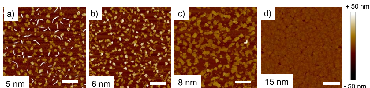
Figure 3. AFM height images of DNTT thin films of thicknesses of (a) 5 nm, (b) 6 nm, (c) 8 nm and (d) 15 nm. Scale bar: 2 \mu\text{m} .
