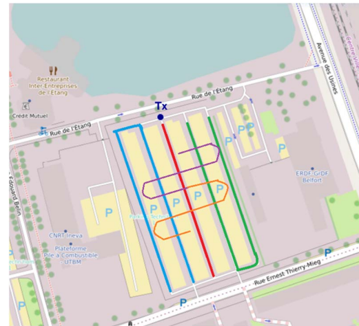
Fig. 5. Overview of measurements area with Tx position and Rx routes
