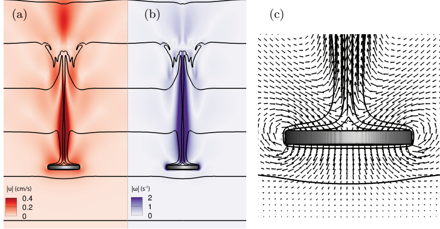
FIGURE 4. Colormaps of (a) velocity |u| and (b) vorticity |\omega| fields for run N12. (c) Zoom on the velocity vector field around the disk. Black solid lines are isopycnals for \rho equals 1017.5kg/cm 3 to 1020.6kg/cm 3 by step of 0.5kg/cm 3 . In (c), isopycnals with \rho = 1017.5\text{kg/cm}^3 and \rho = 1020.6\text{kg/cm}^3 are not visible. The images correspond to U = 0.18\text{cm/s} .
