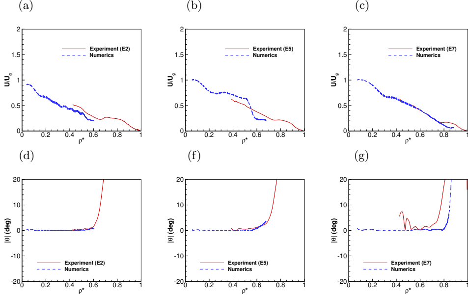
FIGURE 15. Comparison of numerical simulations Nv5, 6, and 7 with experimental runs E2, 5 and 7 respectively, in terms of velocity (a-c) and orientation angle of the disk (e-g) as a function of the normalized fluid density \rho^* .
