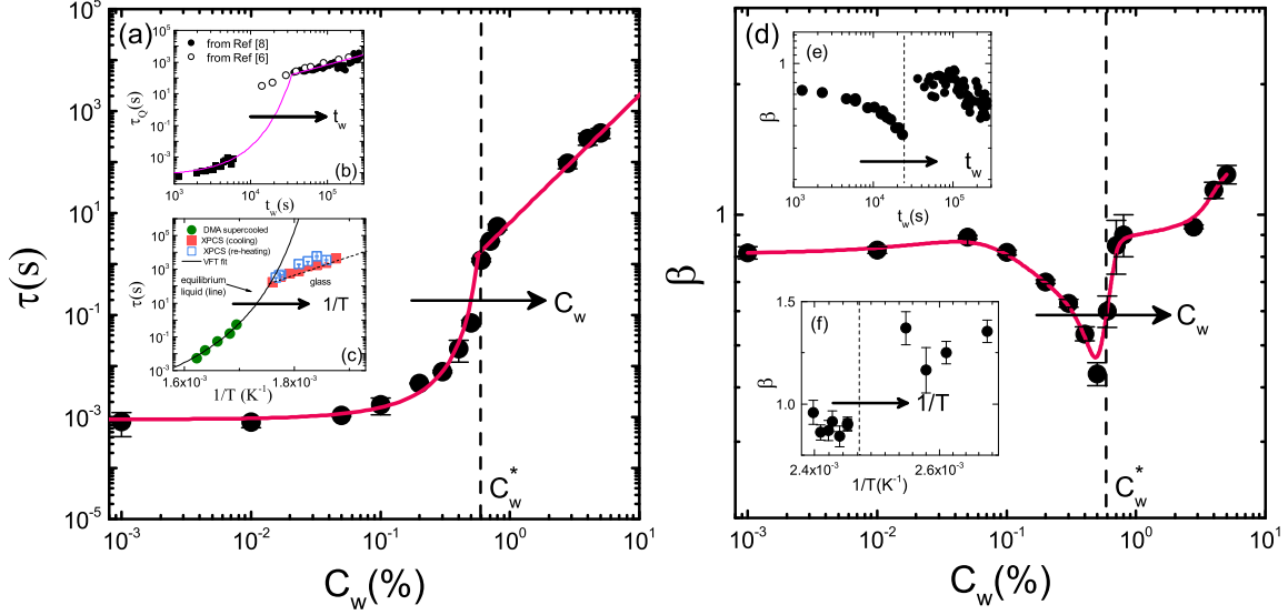
Figure 3: (a) Structural relaxation time from Eq.(1) as a function of weight concentration for IPN microgel suspensions at C_{PAAc}=24.6 %, T=311 K and Q=0.022 nm ^{-1} . Full lines represent the best fits with Eq.(2) and power law behaviours at small and large C_w respectively. (b) Structural relaxation time behaviour with aging time t_w from Ref. (6) for colloidal suspensions of Laponite and (c) structural relaxation time behaviour with the inverse of temperature 1/T from Ref. (17) for a metallic glass. (d) \beta parameter from Eq.(1) as a function of weight concentration for IPN microgel suspensions. Full line is a guide to eyes. (e) \beta exponent as a function of aging time t_w from Ref. (6, 53) for colloidal suspensions of Laponite and (f) \beta exponent dependence with 1/T from Ref. (16) for a metallic glass.
