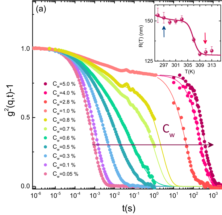
Figure 1: (a) Normalized intensity autocorrelation functions of IPN microgel particles at C_{PAAc} = 24.6\% , T = 311 K and Q = 0.022 \text{ nm}^{-1} as a function of concentration and (b) Temperature behaviour of the hydrodynamic radius at C_w = 0.01\% , blue and red arrows indicate T = 297 K and T = 311 K respectively.
