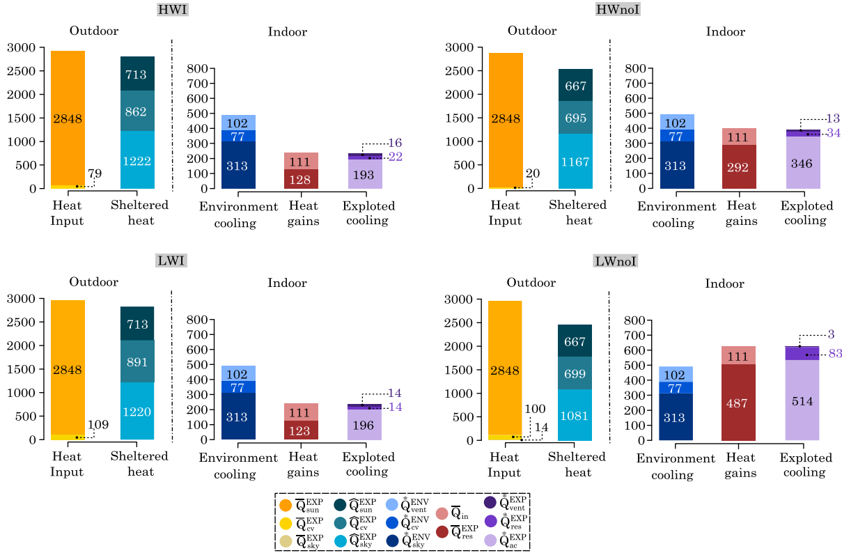
Fig. 4.7. Comparison between the annual ERIs and BPIs (kWh.m 2 .an -1 ) for the four envelope compositions.
