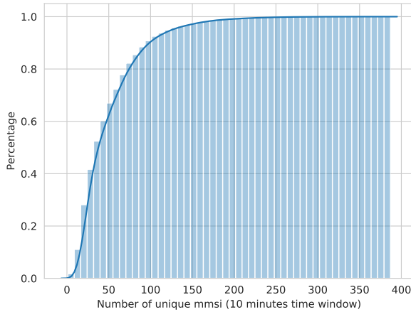
Fig. 10. CDF of the number of unique MMSIs received in a 10 minutes time window for the original dataset (2011-2018). Reading: 80% of the time less than 80 unique MMSIs are received on a 10 minutes time window.
