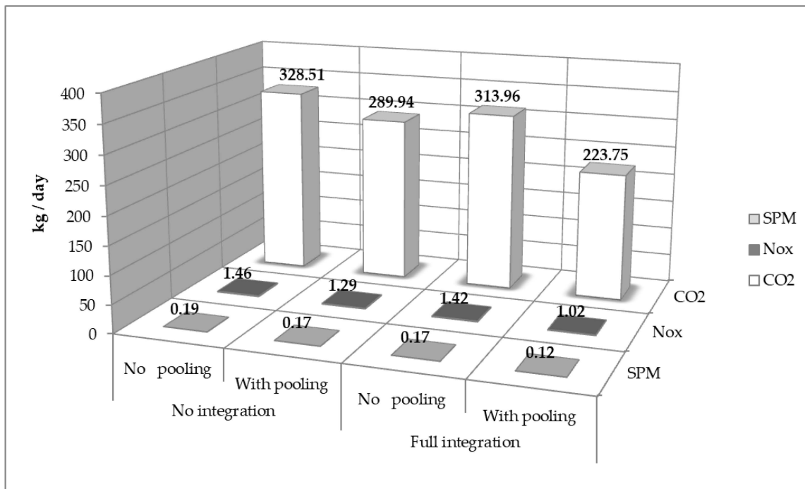
Figure 7. Emissions: CO 2 , NO x , SPM—Heterogeneous fleet (HT).
