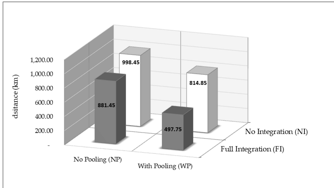
Figure 4. Total cumulated distances (TD)—Homogeneous fleet (HM).
