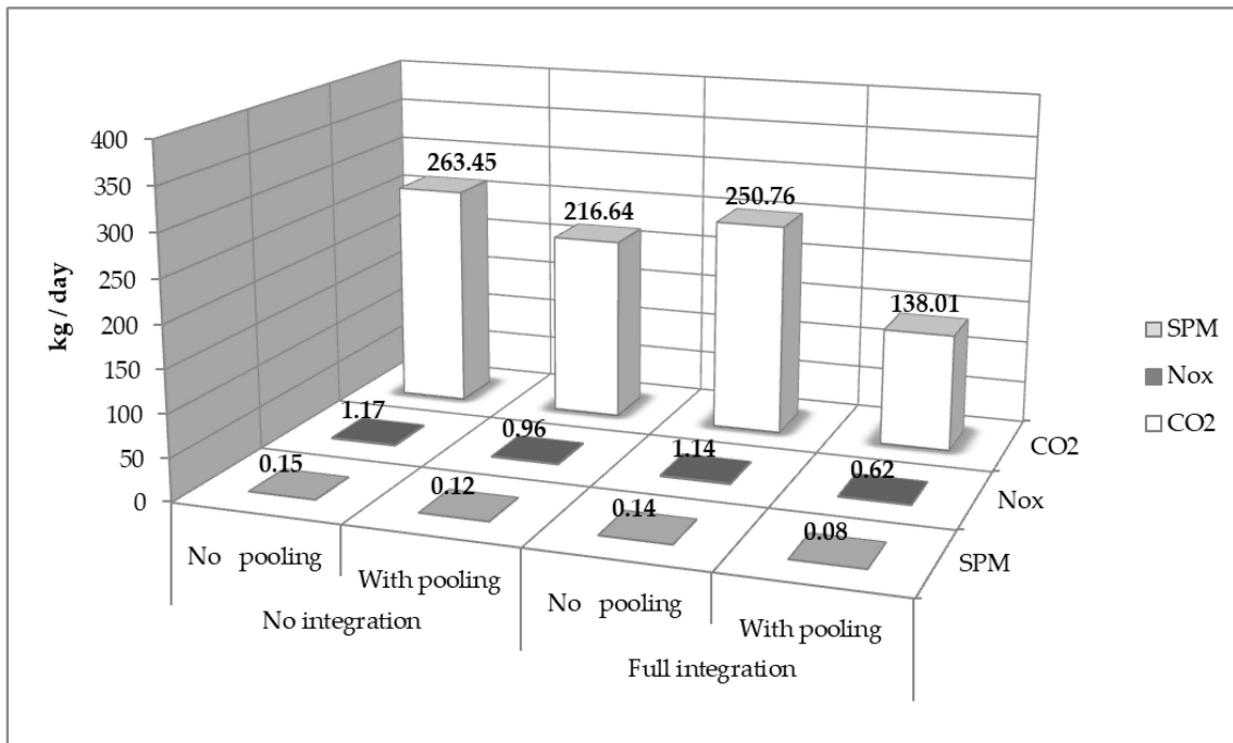
Figure 6. Emissions: CO 2 , NO x , suspended particulate matter (SPM)—Homogeneous fleet (HM).
