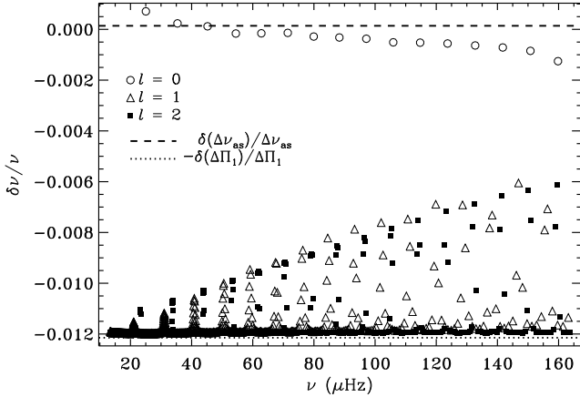
Fig. 9. Relative differences in computed frequencies for the MESA solar-calibrated 1.5 M_\odot, 7 R_\odot model, compared with the ASTEC results, in the sense (MESA) - (ASTEC), for l = 0 (open circles), l = 1 (open triangles) and l = 2 (filled squares). The differences are evaluated at fixed radial order.
