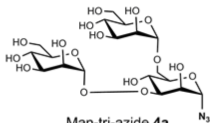
Man-tri-azide 4a
