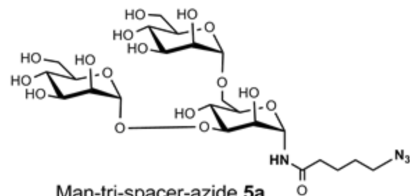
Man-tri-spacer-azide 5a
