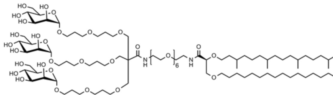
Tri-Man-diether 1
