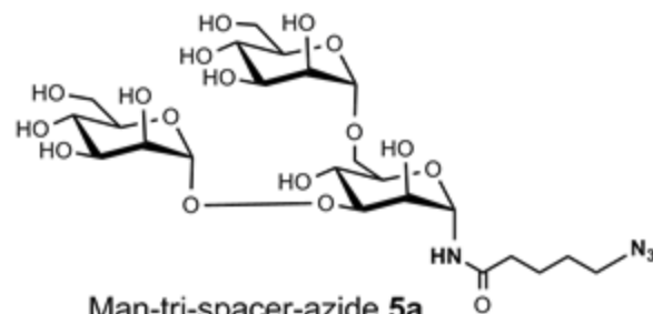
Man-tri-spacer-azide 5a
