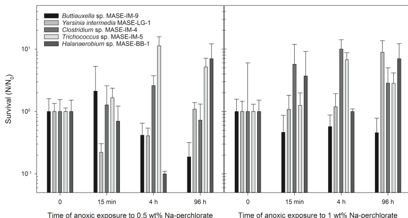
Figure 2. Response of organisms to Na-perchlorate. MASE-strain cultures ( Buttiauxella sp. MASE-IM-9, Yersinia intermedia MASE-LG-1, Clostridium sp. MASE-IM-4, Trichococcus sp. MASE-IM-5, Halanaerobium sp. MASE-BB-1) were incubated in the presence of Na-perchlorate under anoxic conditions at room temperature. N_0 : Viable cells without added perchlorate, N : Viable cells after storage in the presence of perchlorates (0.5 wt% or 1.0 wt%). Recovery was performed under standard cultivation conditions without perchlorate ( n=3 ). Error bars are representing the standard deviation.
