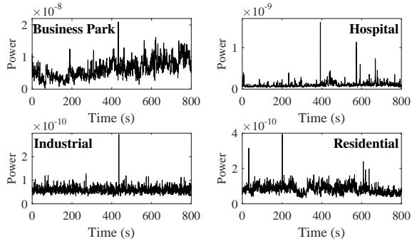
Fig. 2. Example of interference samples measured in the different areas.
