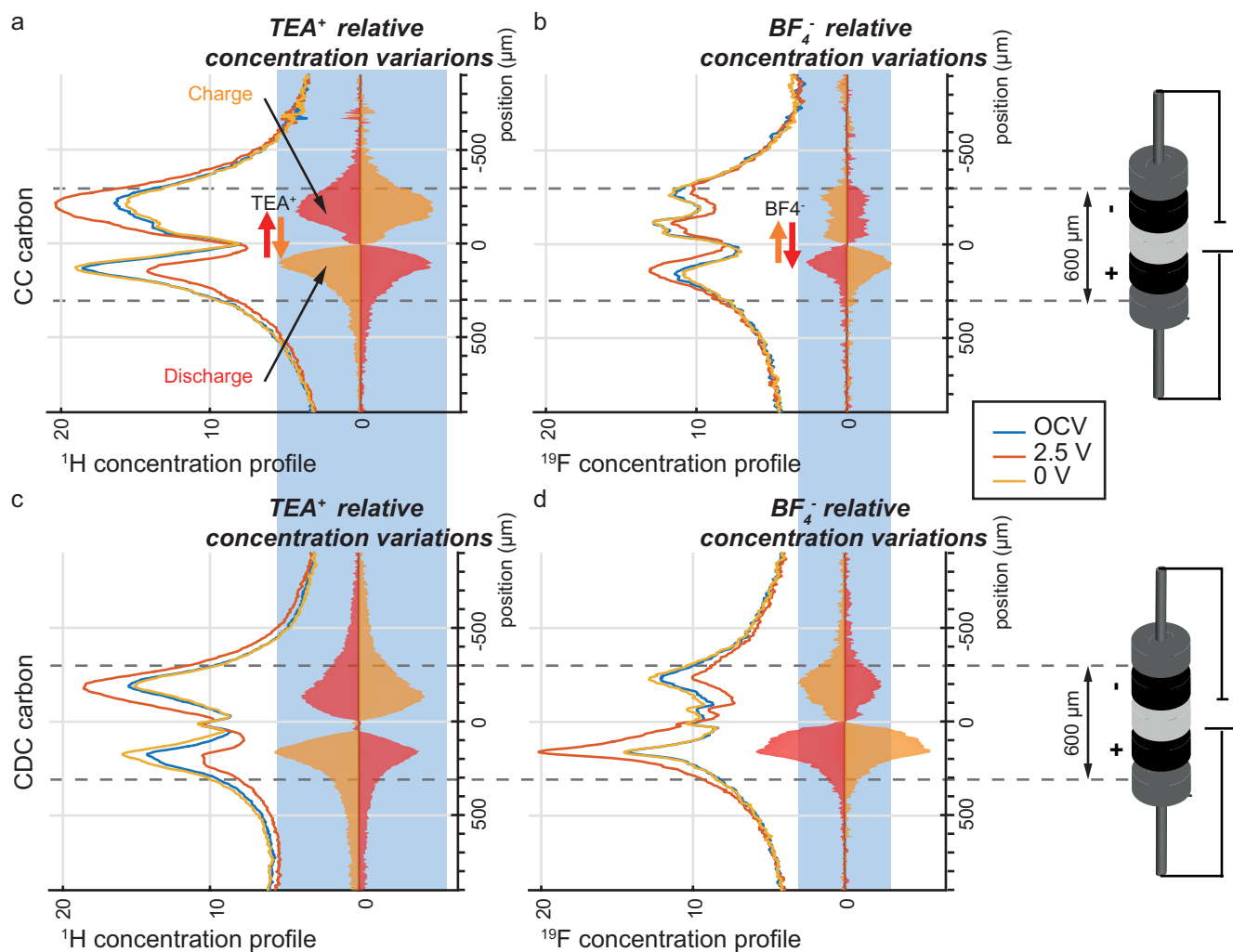
Figure S7. ^1\text{H} (a,c) and ^{19}\text{F} (b,d) 1D concentration profiles of a supercapacitor made of CC (a,b) and CDC (c,d) carbons, during OCV before charging (blue), at 2.5 V (red) and 0 V (yellow). The concentration variations on charge (between 2.5 V and OCV) are displayed on the right of the profiles as filled red curves, and the concentration changes on discharge (between 2.5 V and 0 V) are displayed as filled orange curves.
