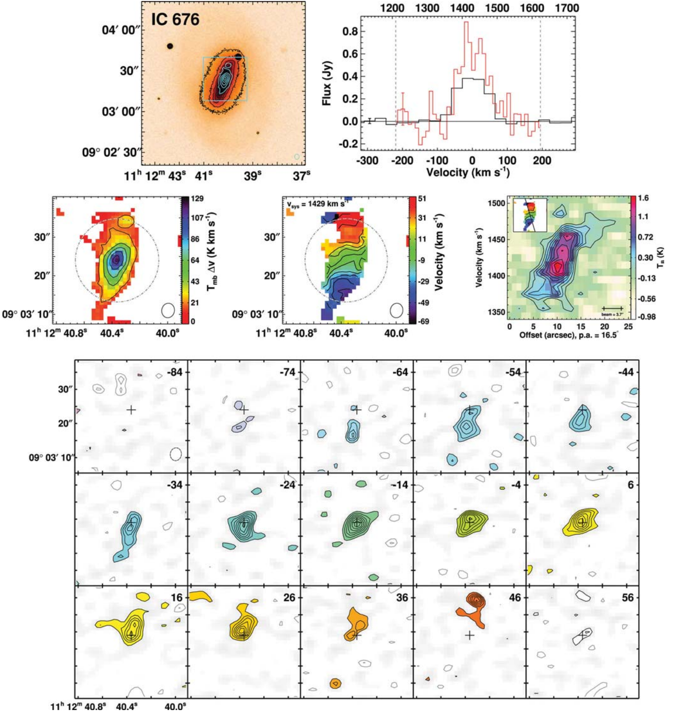
Figure A1. IC 676 is a field regular rotator ( M_K = -22.27 ) with a bar and ring stellar morphology. It has a dust filament. The moment0 peak is 17 Jy beam -1 km s -1 . The moment1 contours are placed at 10 km s -1 intervals and the PVD contours are placed at 1.5 \sigma intervals.
