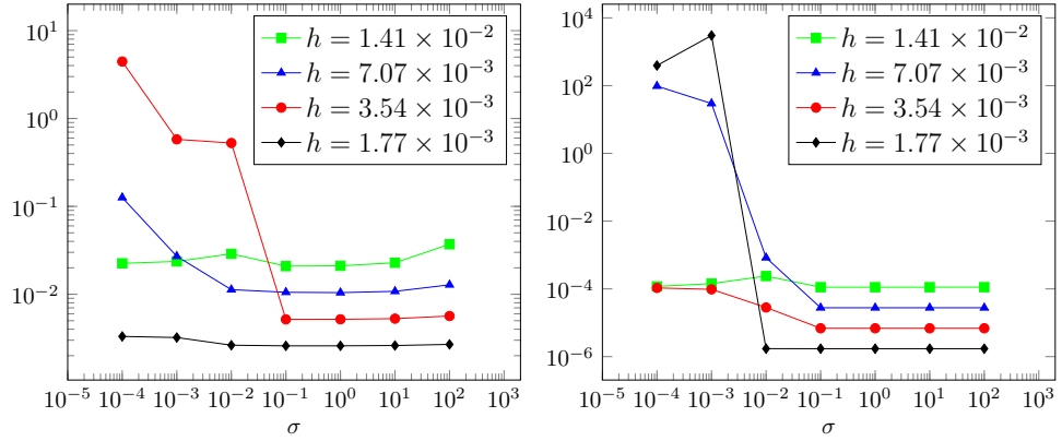
Figure 4: Influence of the ghost penalty parameter \sigma on the relative error |u - u_h|_{1,\Omega} / |u|_{1,\Omega} for \phi -FEM in the 1 st test case. Left: k = 1 ; Right: k = 2 .
