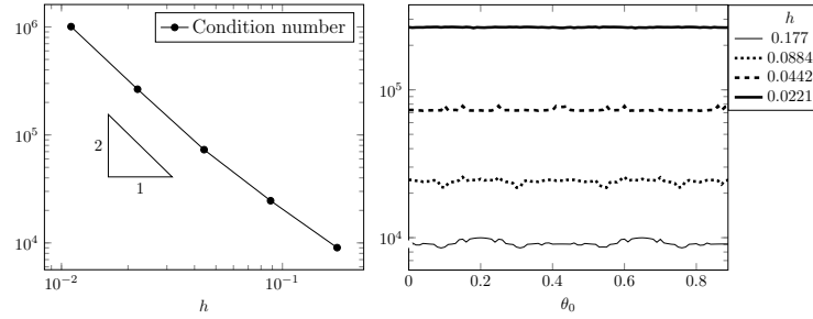
Figure 8: Condition number in \phi -FEM for the test case 1, \sigma = 0.01 , \gamma_u = \gamma_p = \gamma_{\text{div}} = 10 , \theta_0 = 0 , k = 1 and l = k + 2 . Left: \theta_0 = 0 ; Right: different values of \theta_0 .
