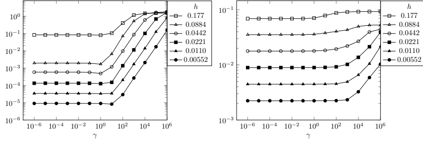
Figure 7: Sensitivity of the relative error in \phi -FEM with respect to \gamma_u = \gamma_p = \gamma_{\text{div}} = \gamma with \sigma = 0.01 fixed for the test case 1, \theta_0 = 0 , k = 1 and l = 3 . Left: L^2 relative error; Right: H^1 relative error.
