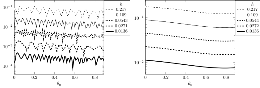
Figure 12: Sensitivity of the relative error with respect to \theta_0 in CutFEM for the test case 2, \sigma = 0.01 . Left: L^2 relative error \|u - u_h\|_{0,\Omega_h^i} / \|u\|_{0,\Omega_h^i} ; Right: H^1 relative error \|u - u_h\|_{1,\Omega_h^i} / \|u\|_{1,\Omega_h^i} .
