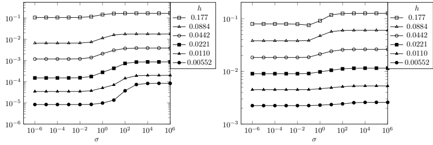
Figure 6: Sensitivity of the relative error in \phi -FEM with respect to \sigma with \gamma_u = \gamma_p = \gamma_{\text{div}} = 10 being fixed for the test case 1, \theta_0 = 0 , k = 1 and l = 3 . Left: L^2 relative error; Right: H^1 relative error.
