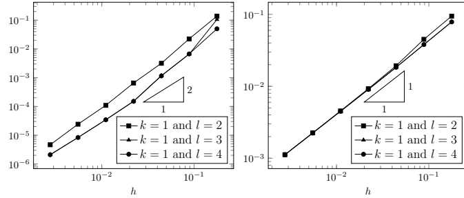
Figure 2: \phi -FEM for the test case 1, \theta_0 = 0 , \sigma = 0.01 and \gamma_u = \gamma_p = \gamma_{\text{div}} = 10 , k = 1 and different values of l . Left: L^2 relative error \|u - u_h\|_{0, \Omega_h^i} / \|u\|_{0, \Omega_h^i} ; Right: H^1 relative error \|u - u_h\|_{1, \Omega_h^i} / \|u\|_{1, \Omega_h^i} .
