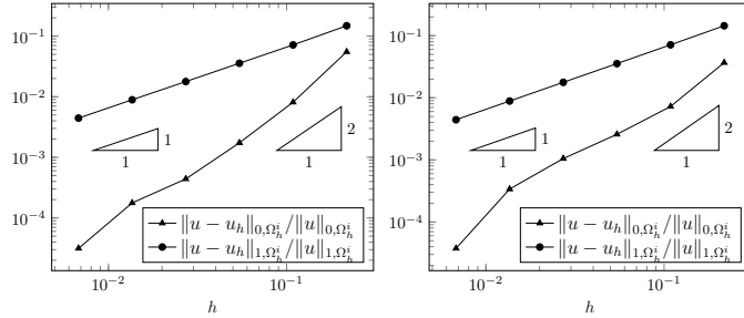
Figure 10: L^2 and H^1 relative error for the test case 2. Left: \phi -FEM with \sigma = 0.01 , \gamma_u = \gamma_p = \gamma_{\text{div}} = 10 , k = 1 and l = 3 ; Right: CutFEM, \theta_0 = \pi/8 , \sigma = 0.01 .
