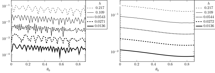
Figure 12: Sensitivity of the relative error with respect to \theta_0 in CutFEM for the test case 2, \sigma = 0.01 . Left: L^2 relative error \|u - u_h\|_{0, \Omega_h^i} / \|u\|_{0, \Omega_h^i} ; Right: H^1 relative error \|u - u_h\|_{1, \Omega_h^i} / \|u\|_{1, \Omega_h^i} .
