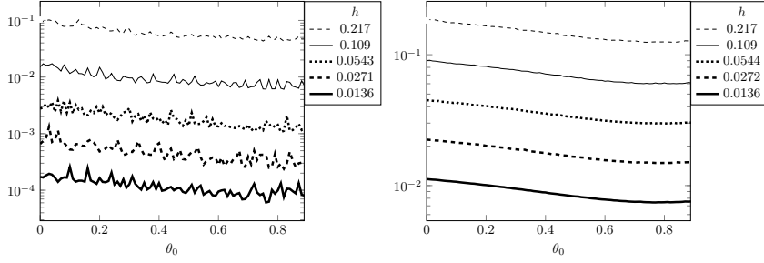
Figure 11: Sensitivity of the relative error with respect to \theta_0 in \phi -FEM for the test case 2, \sigma = 0.01 , \gamma_u = \gamma_p = \gamma_{\text{div}} = 10 , k = 1 and l = 3 . Left: L^2 relative error \|u - u_h\|_{0, \Omega_h^i} / \|u\|_{0, \Omega_h^i} ; Right: H^1 relative error \|u - u_h\|_{1, \Omega_h^i} / \|u\|_{1, \Omega_h^i} .
