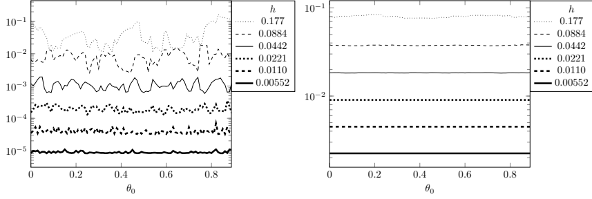
Figure 5: Sensitivity of the relative error with respect to \theta_0 in \phi -FEM for the test case 1, \sigma = 0.01 and \gamma_u = \gamma_p = \gamma_{\text{div}} = 10 , k = 1 and l = 3 . Left: L^2 relative error \|u - u_h\|_{0, \Omega_h^i} / \|u\|_{0, \Omega_h^i} ; Right: H^1 relative error \|u - u_h\|_{1, \Omega_h^i} / \|u\|_{1, \Omega_h^i} .
