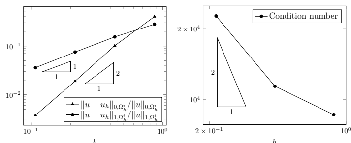
Figure 13: \phi -FEM for the test case 3, \sigma = 0.01 , \gamma_u = \gamma_p = \gamma_{\text{div}} = 10 , k = 1 and l = 3 . Left: L^2 and H^1 relative error; Right: condition number.
