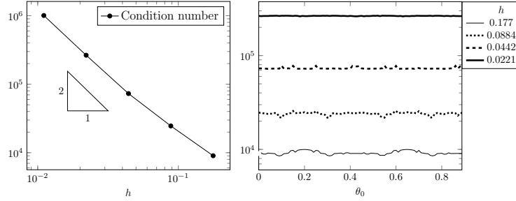
Figure 8: Condition number in \phi -FEM for the test case 1, \sigma = 0.01 , \gamma_u = \gamma_p = \gamma_{div} = 10 , \theta_0 = 0 , k = 1 and l = k + 2 . Left: \theta_0 = 0 ; Right: different values of \theta_0 .
