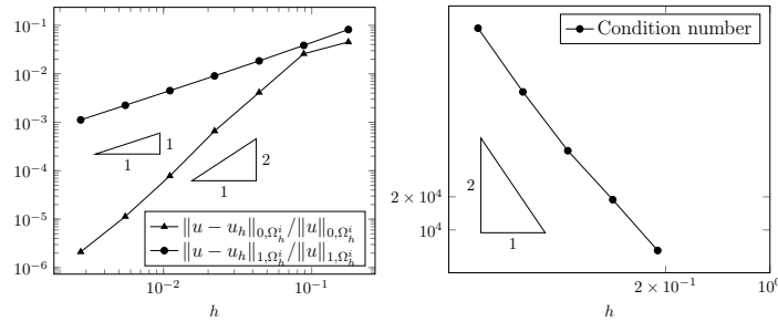
Figure 9: \phi -FEM for the test case 1 and Robin boundary conditions, \sigma = 0.01 , \gamma_u = \gamma_p = \gamma_{div} = 10 , \alpha = 1 , k = 1 and l = 3 . Left: L^2 relative error \|u - u_h\|_{0,\Omega_h^i} / \|u\|_{0,\Omega_h^i} and H^1 relative error \|u - u_h\|_{1,\Omega_h^i} / \|u\|_{1,\Omega_h^i} ; Right: Condition number.
