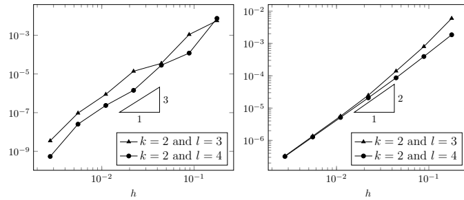
Figure 3: \phi -FEM for the test case 1, \theta_0 = 0 , \sigma = 0.01 , \gamma_u = \gamma_p = \gamma_{\text{div}} = 10 , k = 2 and different values of l . Left: L^2 relative error \|u - u_h\|_{0,\Omega_h^i} / \|u\|_{0,\Omega_h^i} ; Right: H^1 relative error \|u - u_h\|_{1,\Omega_h^i} / \|u\|_{1,\Omega_h^i} .
