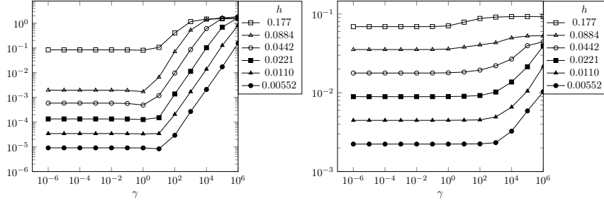
Figure 7: Sensitivity of the relative error in \phi -FEM with respect to \gamma_u = \gamma_p = \gamma_{div} = \gamma with \sigma = 0.01 fixed for the test case 1, \theta_0 = 0 , k = 1 and l = 3 . Left: L^2 relative error; Right: H^1 relative error.
