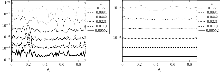
Figure 4: Sensitivity of the relative error with respect to \theta_0 in \phi -FEM for the test case 1, \sigma = 0.01 and \gamma_u = \gamma_p = \gamma_{\text{div}} = 20 , k = 1 and l = 2 . Left: L^2 relative error \|u - u_h\|_{0, \Omega_h^i} / \|u\|_{0, \Omega_h^i} ; Right: H^1 relative error \|u - u_h\|_{1, \Omega_h^i} / \|u\|_{1, \Omega_h^i} .
