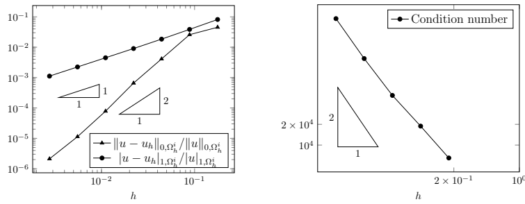
Figure 9: \phi -FEM for the test case 1 and Robin boundary conditions, \sigma = 0.01 , \gamma_u = \gamma_p = \gamma_{\text{div}} = 10 , \alpha = 1 , k = 1 and l = 3 . Left: L^2 relative error \|u - u_h\|_{0,\Omega_h^i} / \|u\|_{0,\Omega_h^i} and H^1 relative error \|u - u_h\|_{1,\Omega_h^i} / \|u\|_{1,\Omega_h^i} ; Right: Condition number.
