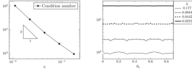
Figure 8: Condition number in \phi -FEM for the test case 1, \sigma = 0.01 , \gamma_u = \gamma_p = \gamma_{\text{div}} = 10 , \theta_0 = 0 , k = 1 and l = k + 2 . Left: \theta_0 = 0 ; Right: different values of \theta_0 .
