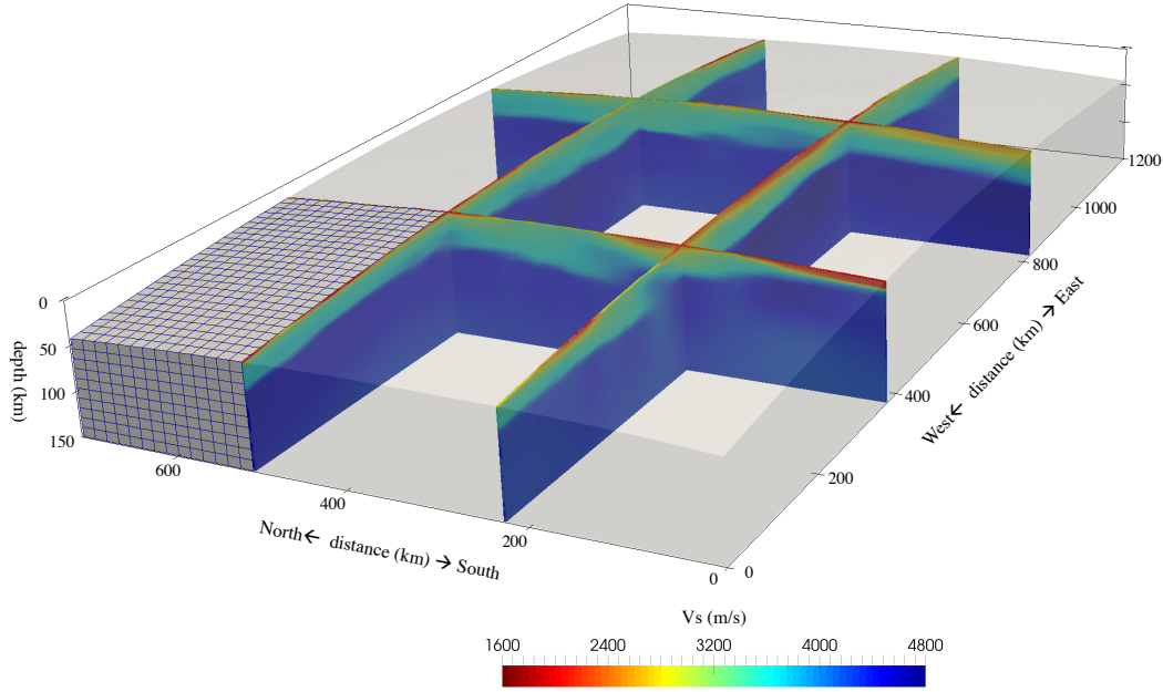
Figure 2. Mesh and shear-wave velocity of the initial model. The gray volume indicates the scope of the initial model. It is centered at [11^\circ\text{E}, 46^\circ\text{N}] with lateral dimensions 1200 km in the East-West direction and 720 km in the North-South direction. We show shear-wave velocity values of the initial model in four representative depth-sections. We show a chunk of the mesh for the North-West portion of the initial model. The topography and curvature of the Earth are accounted by vertically deforming the mesh grid.
