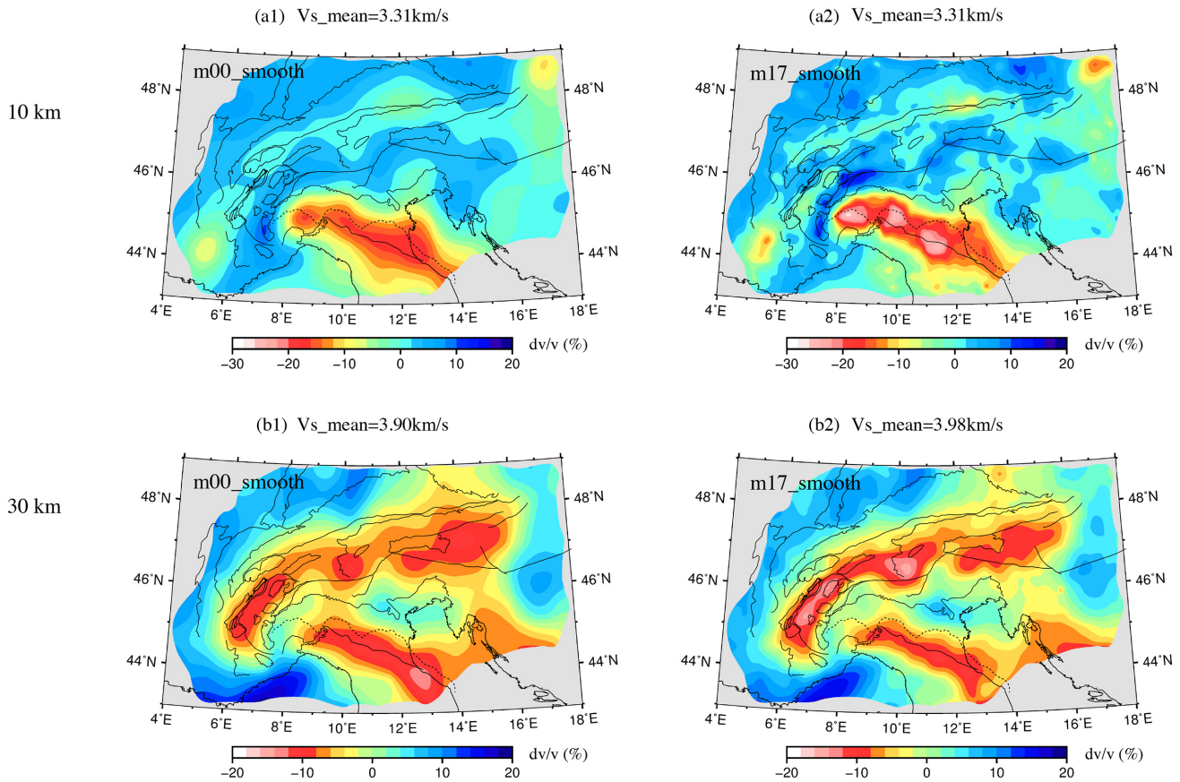
Figure 10. V_s depth slices at 10 and 30 km in the smooth initial model (m00_smooth; a1 and b1) and the corresponding final model (m17_smooth; a2 and b2). As in Fig. 8, we display the relative variations of velocity with respect to the average velocity in the depth slice, and we discard areas with poor data coverage.
