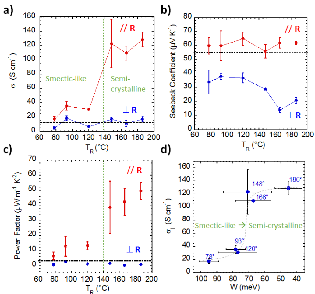
Figure 4: Evolution of the a) charge conductivity, b) Seebeck Coefficient, and c) power factor measured along ( // R) or perpendicular ( \perp R) to the rubbing direction for P3HT films rubbed at different temperatures and doped with F 4 TCNQ (1 mg/ml). The black dashed lines represent the values for a non-oriented sample. The error bars are mainly related to the statistic dispersion in alignment level of samples. In a and c, the vertical green lines are a guide for the eye to differentiate the ranges of smectic-like and semi-crystalline phases. d) Evolution of the charge conductivity \sigma_{||}
