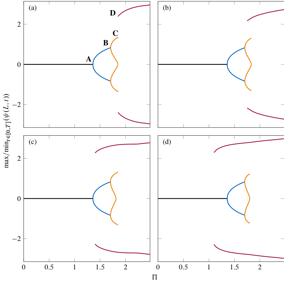
Figure 12: Bifurcation diagrams for a two-dimensional inverted flag with different mass ratios: (a) \mu = 0.1 , (b) \mu = 0.5 , (c) \mu = 2.0 , and (d) \mu = 5.0 , indicating the minimum and maximum values of the leading edge rotation over a cycle of steady-state oscillation of period T^* . [—] Stable static solution (undeflected stable equilibria); [—] stable static solutions (deflected static equilibria) corresponding to buckling of the inverted flag to either side; [—] stable periodic solutions (oscillation around deflected equilibria) corresponding to deformed-flapping of the inverted flag to either side; [—] stable periodic solution (oscillations around undeflected equilibrium). Colour scheme as in figure 6.
