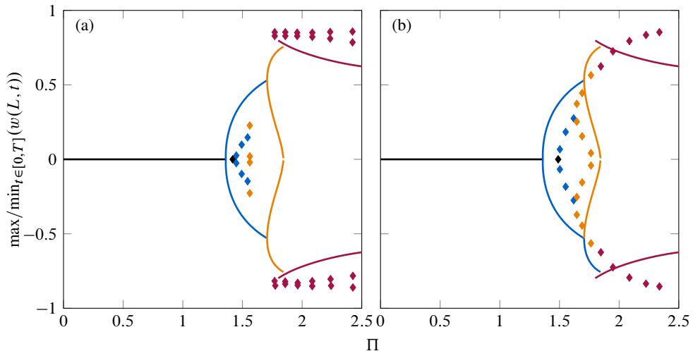
Figure 19: Bifurcation diagrams for inverted flags with \mu = 0.2 over a cycle of period T^* steady-state oscillation. [—] stretched-straight state; [—] buckled state; [—] deformed-flapping regime; and [—] large-amplitude flapping around the origin. Lines show the results obtained by the present model, while symbols [◆], [◆], and [◆] show the corresponding results obtained by Goza et al. (2018) . (a) Re = 200 , and (b) Re = 20 .
