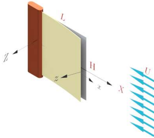
Figure 1: Two-dimensional inverted flag in axial flow: free at the upstream and clamped at the downstream end. The flag is assumed to be infinitely wide (i.e. H/L \rightarrow \infty ); hence, the fluid flow surrounding the flag is treated as two-dimensional.
