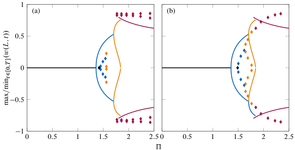
Figure 19: Bifurcation diagrams for inverted flags with \mu = 0.2 over a cycle of period T^* steady-state oscillation. [—] stretched-straight state; [—] buckled state; [—] deformed-flapping regime; and [—] large-amplitude flapping around the origin. Lines show the results obtained by the present model, while symbols [◆], [◆], and [◆] show the corresponding results obtained by Goza et al. (2018) . (a) Re = 200 , and (b) Re = 20 .
