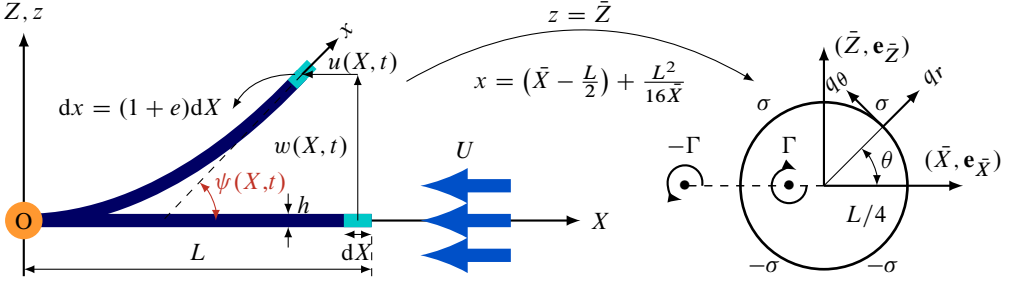
Figure 2: (Left) The flag is idealised as an inextensible (i.e. e = 0 ) cantilevered beam. An arbitrary infinitesimal element dx of the beam undergoes longitudinal u(X, t) and transverse w(X, t) displacements, related to each other by the rotation angle \psi(X, t) . (Right) Joukowski's conformal mapping of the plate into a circle of radius L/4 (i.e. \bar{X}\bar{Z} -plane); q_r and q_\theta are the radial and circumferential velocities on the circle in the \bar{X}\bar{Z} -plane, respectively. The impermeability condition is satisfied by considering a set of sources and sinks of strength \sigma on the top and bottom halves of the circle, respectively. The induced velocity due to a single bound vortex of strength \Gamma and its image (i.e. the wake vortex of strength -\Gamma ) at an arbitrary point on the circle satisfies the Kutta condition.
