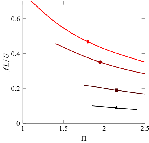
Figure 13: Sensitivity of the large-amplitude flapping reduced frequency to the dimensionless flow velocity \Pi for inverted flags of different mass ratios: [ \blacktriangle ] \mu = 0.1 ; [ \blacksquare ] \mu = 0.5 ; [ \bullet ] \mu = 2.0 ; and [ \blacklozenge ] \mu = 5.0 .
