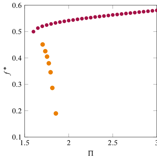
Figure 10: Dimensionless frequency f^* versus dimensionless flow velocity \Pi for an inverted flag with \mu = 1.0 . Colour scheme as in figure 6.
