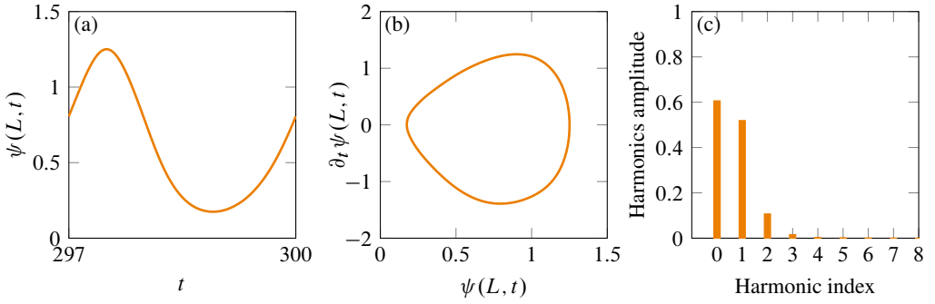
Figure 8: Response of the inverted flag, with \mu = 1.0 at \Pi = 1.80 , displaying a periodic motion around the deflected equilibrium; (a) time history, (b) phase portrait, and (c) the frequency content of the response, obtained from FFT. Colour scheme as in figure 6.
