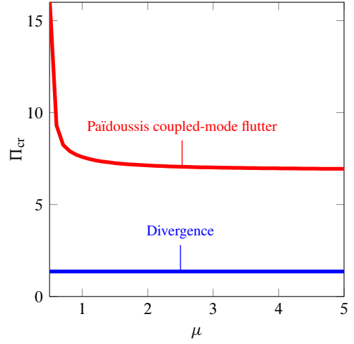
Figure 5: Stability map for a 2D inverted flag; [—]: the onset of divergence, [—]: the onset of flutter.
