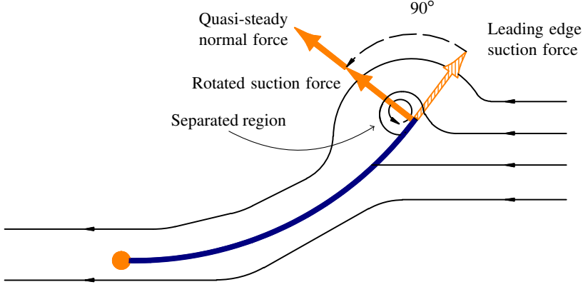
Figure 3: Flow around the 2D inverted flag placed in an inviscid fluid. The Kutta condition enforces a smooth, tangential flow leaving the trailing edge. However, according to Polhamus’s leading edge suction analogy, the leading edge suction vanishes due to separation at the leading edge, and it forms a leading edge vortex. This results in a normal force component of equal magnitude to the leading edge suction. Effectively, the leading edge suction force is rotated by 90^\circ onto the low-pressure side of the flag.
