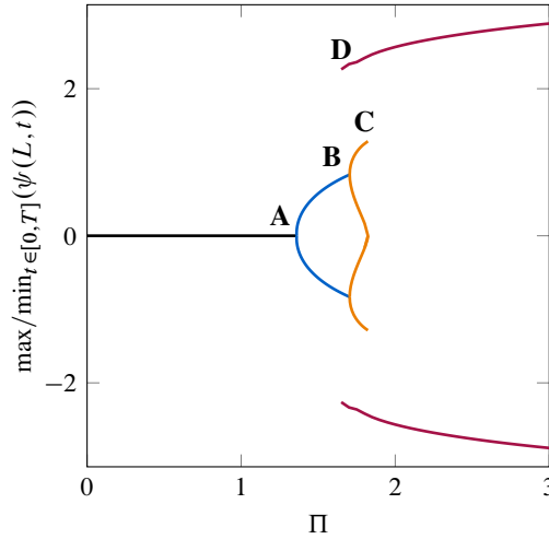
Figure 6: Bifurcation diagram for a two-dimensional inverted flag with \mu = 1.0 , indicating the minimum and maximum values of the leading edge rotation over a cycle of steady-state oscillation of period T^* . [—] Undeflected stable equilibrium; [—] deflected stable equilibrium corresponding to buckling of the inverted flag to either side; [—] stable periodic solutions (oscillation around deflected equilibria) corresponding to deformed-flapping of the inverted flag to either side; [—] stable periodic solution (oscillations around undeflected equilibrium). This colour scheme is also utilized in figures 7-10.
