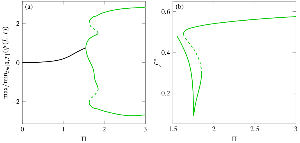
Figure 15: Nonlinear response of a two-dimensional inverted flag with \mu = 1.0 and \psi_0 = 0.1 . (a) Bifurcation diagram indicating the minimum and maximum values of the leading edge rotation over a cycle of steady-state oscillation of period T^* : [—] Stable static solution; [---] unstable and [—] stable periodic solution (asymmetric oscillations). (b) Dimensionless frequency f^* versus dimensionless flow velocity \Pi .
