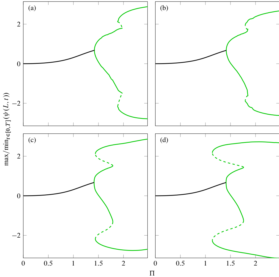
Figure 16: Bifurcation diagrams for \psi_0 = 0.2 and various mass ratios: (a) \mu = 0.1 , (b) \mu = 0.5 , (c) \mu = 2.0 , and (d) \mu = 5.0 , indicating the minimum and maximum values of the leading edge rotation over a cycle of steady-state oscillation of period T^* . [—] Stable static solution; [---] unstable and [—] stable periodic solutions (asymmetric oscillations).
