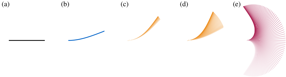
Figure 7: Shapes of the two-dimensional inverted flag studied in figure 6: (a) stretched-straight state ( \Pi = 1.35 ), (b) buckled state ( \Pi = 1.40 ), (c) at the onset of deformed-flapping mode ( \Pi = 1.71 ), (d) deformed-flapping mode ( \Pi = 1.75 ), and (e) large-amplitude flapping ( \Pi = 1.65 ). Colour scheme as in figure 6.
