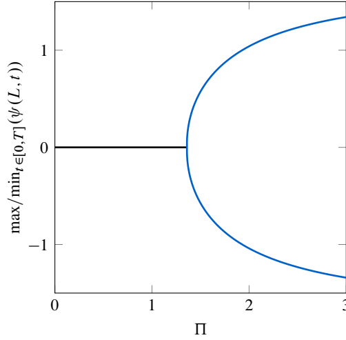
Figure 11: Bifurcation diagram of an inverted flag subjected to steady-fluid forces showing the leading edge rotation angle versus dimensionless flow velocity. [—] Undeflected stable equilibrium and [—] deflected static equilibrium solutions corresponding to buckling of the inverted flag to either side. No secondary bifurcation (dynamic or static) materializes. Colour scheme as in figure 6.
