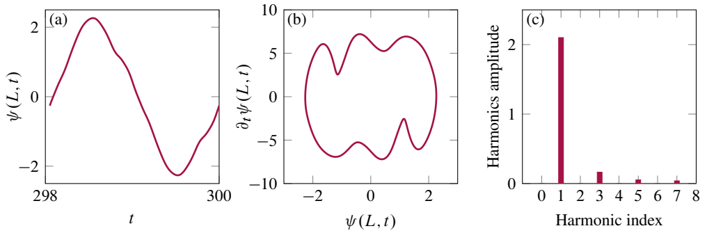
Figure 9: Response of the inverted flag with \mu = 1.0 at \Pi = 1.65 , displaying a periodic motion around the undeflected equilibrium; (a) time history, (b) phase-plane portrait, and (c) the frequency content of the response, obtained from FFT. Colour scheme as in figure 6.
