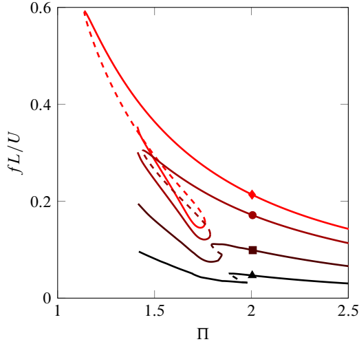
Figure 17: Reduced frequency of the asymmetric flapping motion as a function of the dimensionless flow velocity \Pi for \psi_0 = 0.2 and different mass ratios: \blacktriangle \mu = 0.1 , \blacksquare \mu = 0.5 , \bullet \mu = 2.0 , and \blacklozenge \mu = 5.0 . [-\cdot-\cdot-] Unstable and [-\text{—}] stable periodic solutions.
