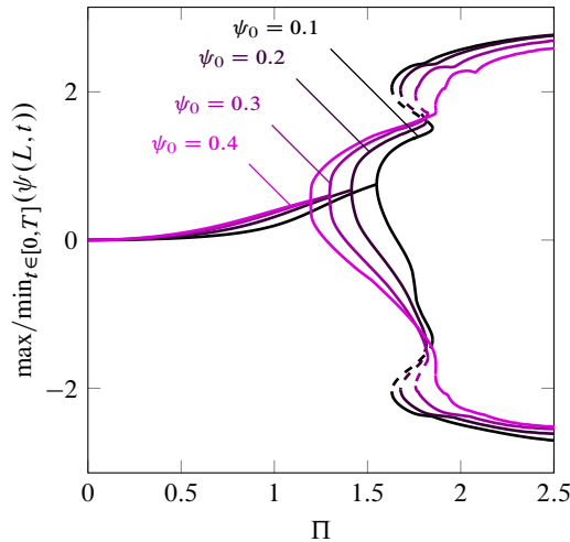
Figure 18: Bifurcation diagram with \mu = 1.0 and various initial angles of attack \psi_0 .
