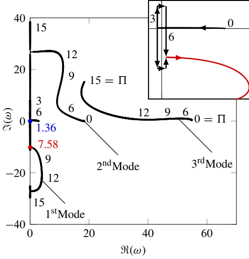
Figure 4: Argand diagram for an inverted flag with \mu = 1.0 , showing the evolution of the first three modes with the dimensionless flow velocity \Pi .
