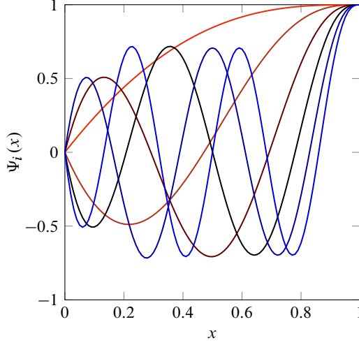
Figure A.1: First six in vacuo comparison functions of a cantilevered beam utilized in the Galerkin discretization of the nonlinear system. First [—], second [—], third [—], fourth [—], fifth [—] and sixth [—] comparison function.
