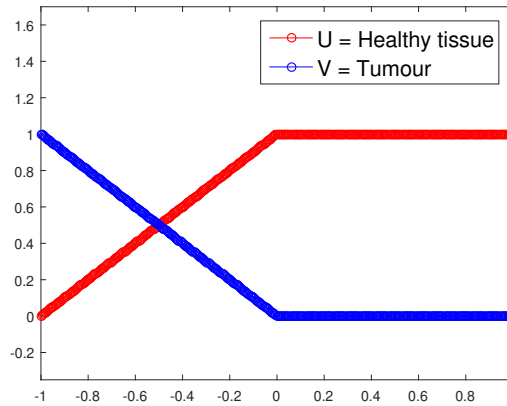
FIGURE 9. Graphs of the initial profiles for the simplified model.
