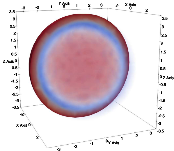
FIGURE 23. Three-dimensional tumour cells density profile located inside the half ball provided with healthy cells density data reproduced throughout the external spherical surface.
