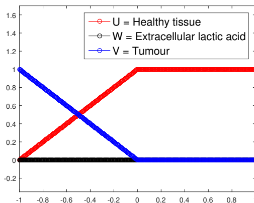
FIGURE 3. Graphs of the initial profiles for the numerical experiments.
