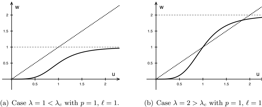
Figure 9: relative positions of the straight line w = u (dotted) and the curve w = \lambda g(u) (continuous) corresponding to different values of \lambda .
