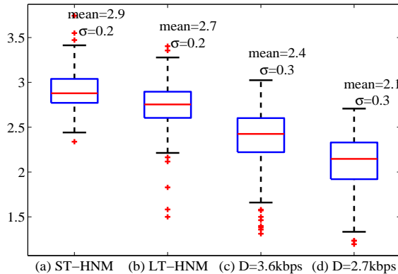
Fig. 14: Listening quality: PESQ scores of TIMIT test database.
