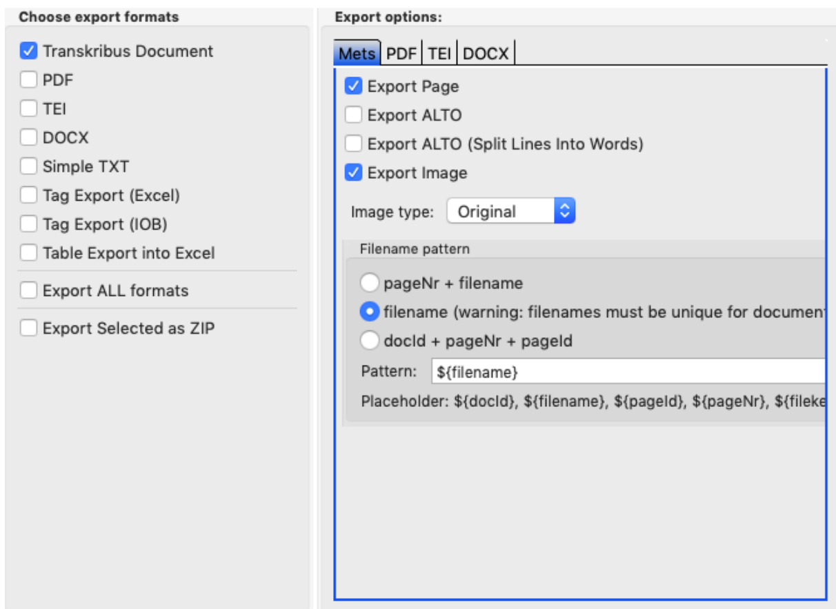
Figure 5. Export formats.
