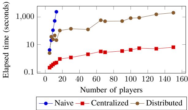
Fig. 3. Running time of the different algorithms with a varying number of players. The y-axis is in log scale.
