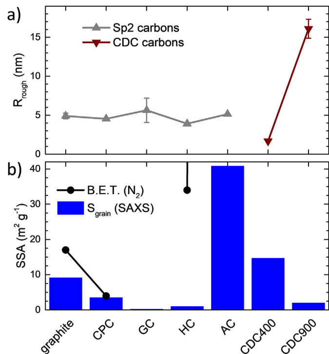
Fig. 8. Morphological refined parameters related to I_{Porod} . a) Characteristic R_{rough} size of the surface roughness of the particles. b) Surface area S_{grain} = S_{macro} + S_{rough} measured from SAXS data (blue columns) and N_2 gas adsorption by the B.E.T. method (black circles). For samples AC, CDC400 and CDC900 the B.E.T. surface area is too large to appear in this graph and can be observed in Fig. 10. (For interpretation of the references to colour in this figure legend, the reader is referred to the Web version of this article.)
