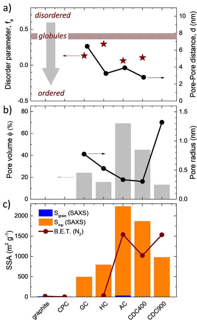
Fig. 10. Microstructural refined parameters related to I_{mp} . a) Disorder parameter (left axis) and pore-pore distance (right axis) of the microporous samples GC, HC, AC and CDC400. b) Micropore volume (left axis) and micropore radius (right axis). c) Specific surface area deduced from SAXS (columns) and gas adsorption (dark red circles). (For interpretation of the references to colour in this figure legend, the reader is referred to the Web version of this article.)
