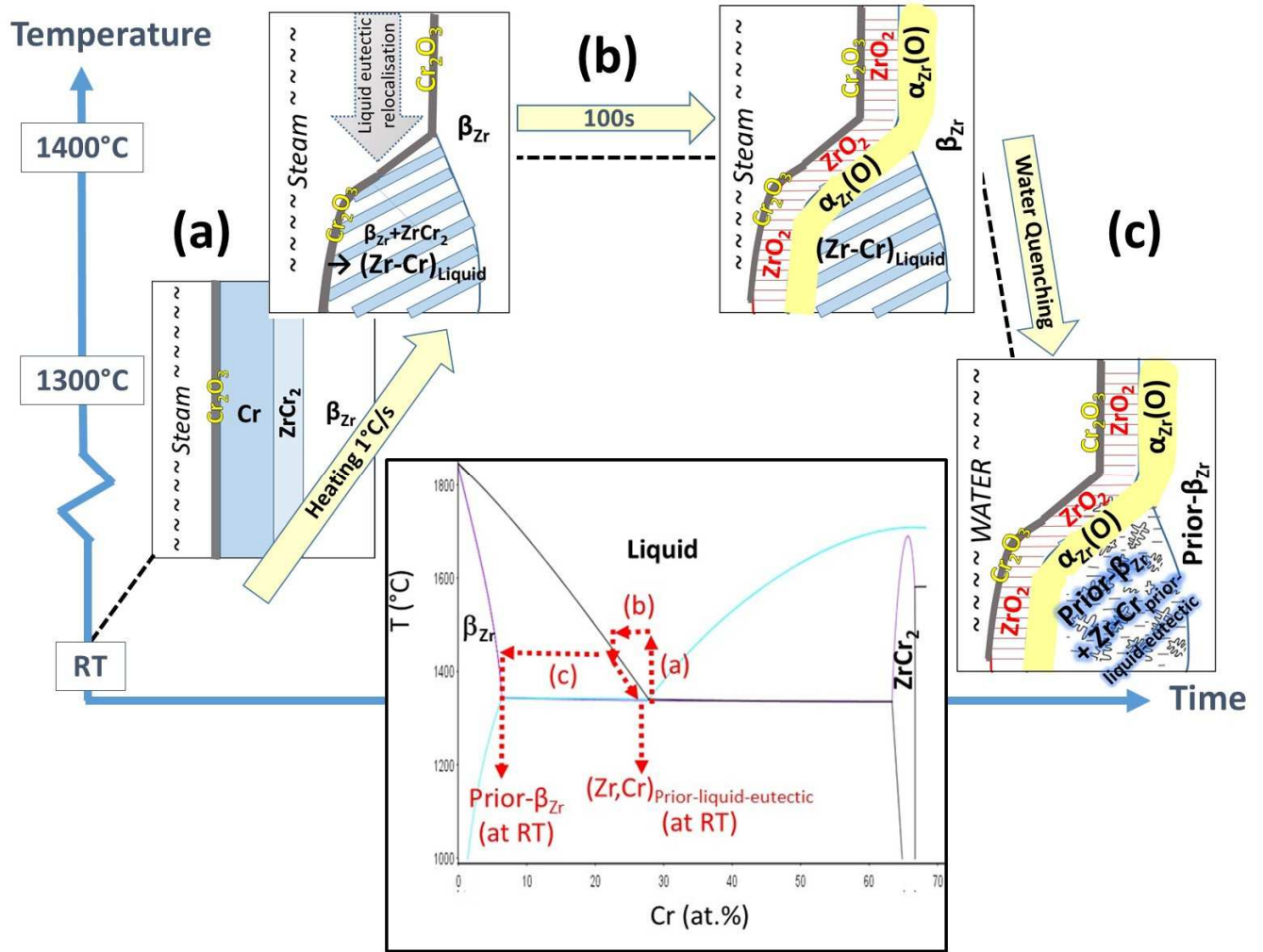
Figure 18 - Phenomenological description of the mechanisms of HT oxidation of Cr-coated M5 Framatome at temperatures above 1300°C, involving eutectic formation and re-solidification; corresponding calculated pseudo-binary M5 Framatome -Cr phase diagram
