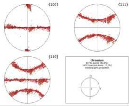
Figure 2 - Typical EBSD orientation maps and associated stereographic pole figures of the first generation 5-10 \mu m-thick Cr-coated Zircaloy-4 (sheet substrate), obtained with different PVD deposition parameters
